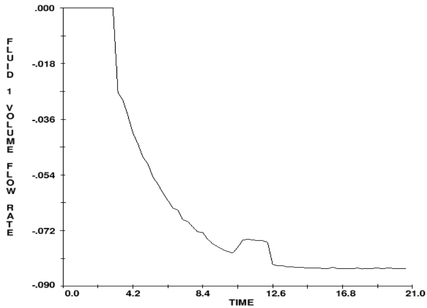
Figure 6.29 Flow Rate Graph for Q=0.50 \text{ m}^3/\text{s} (Intercepted Flow)
