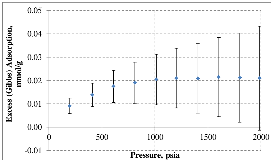
Figure 8.18: Run#5-Methane adsorption isotherm of shale sample A at 50 °C
