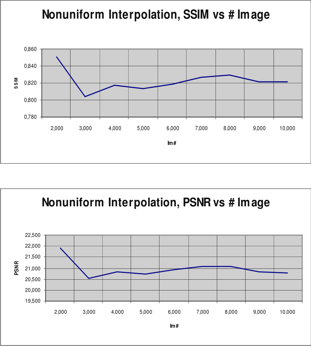
Figure 3.21 Effect of the image quantity on nonuniform interpolation
