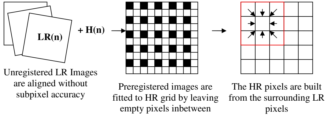
Figure 3.8 Pipeline of Nonuniform Interpolation Algorithm
