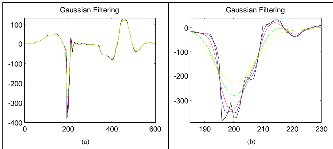
Figure 2.3.8: (Gaussian Filtering). (a) Acceleration Data Results for \sigma=1, 2, 4, 6 , \text{size}=6*\sigma+1 , (b) The samples, between 185 and 230, of Figure 2.3.8.a.
