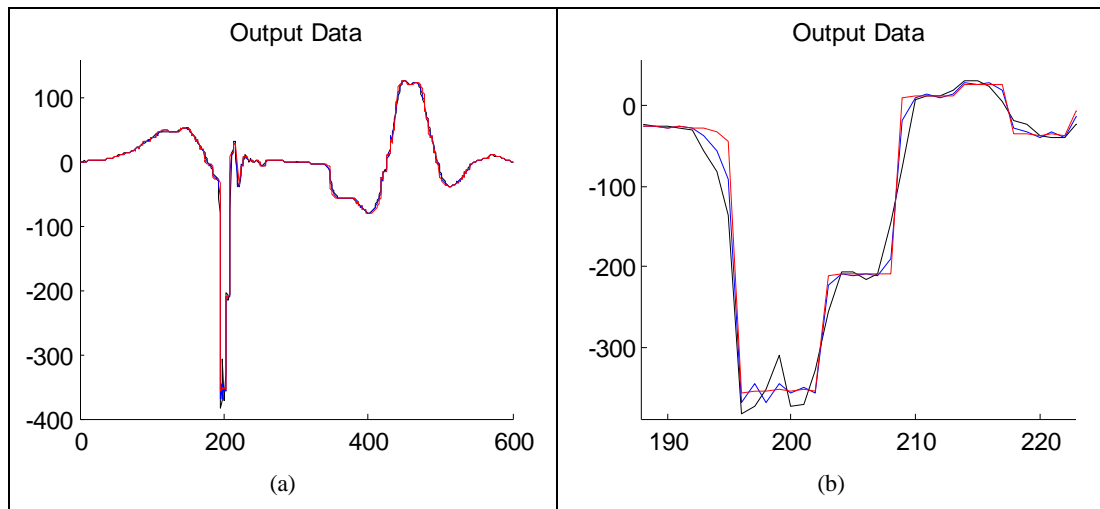
Figure 3.1.3: (Kuwahara Filtering). (a) Smoothed Acceleration Data Result, (b) The samples, between 190 and 220, of Figure 3.1.3.a.
