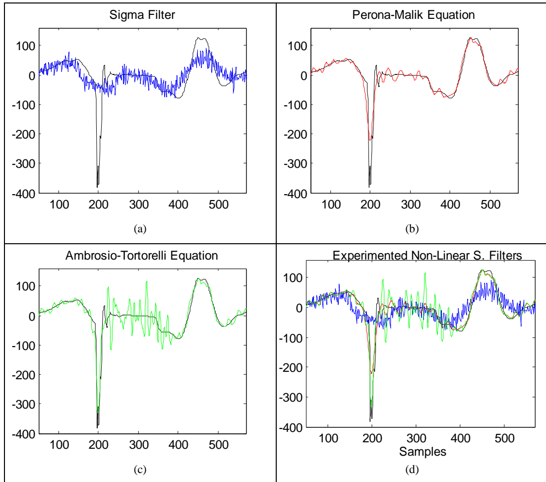
Figure 3.6.4: (The Comparative Second Derivative Results of Displacement Data by using some of the experimented Non-Linear Smoothing Filters). Black Line: Original Acceleration Data, (a) Sigma Filter Result by using \sigma=0.5 , Filter size=91, (b) Perona Malik Filtering Result by using \lambda=10 , T=18 , \Delta t=0.25 and \sigma=3 , (c) Ambrosio Tortorelli Approximation by using T=100 , \Delta t=0.4 , \alpha=8 , \beta=50 , \rho=0.033 , (d) Comparison of all results from Figure 3.6.4.a to Figure 3.6.4.c
