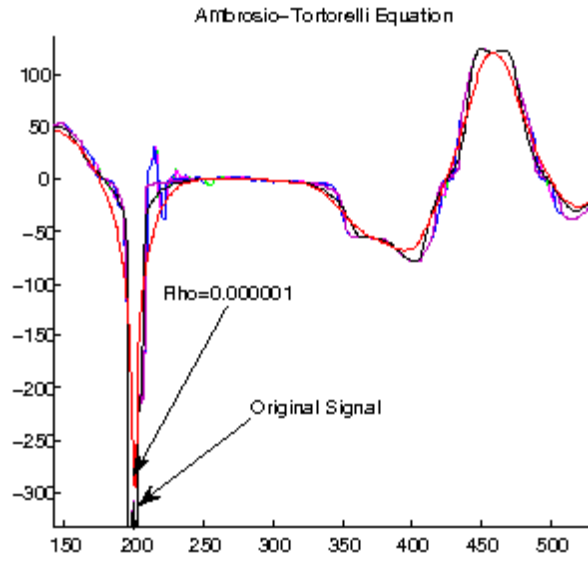
Figure 3.5.3: (Result for the Ambrosio Tortorelli Approximation of the Mumford Shah) The results for T=100 , \Delta t=0.4 , \alpha=32 , \beta=0.4 , \rho=0.05, 0.01, 0.001, 0.0001, 0.00001, 0.000001
