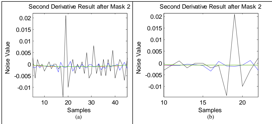
Figure 2.2.4: (Mean Filter vs. Iterated Mean Filter). (a) Second Derivative Result of Smoothed Golf Ball Data using the mask 2, (b) The samples, between 10 and 22, of Figure 2.2.4.a.
