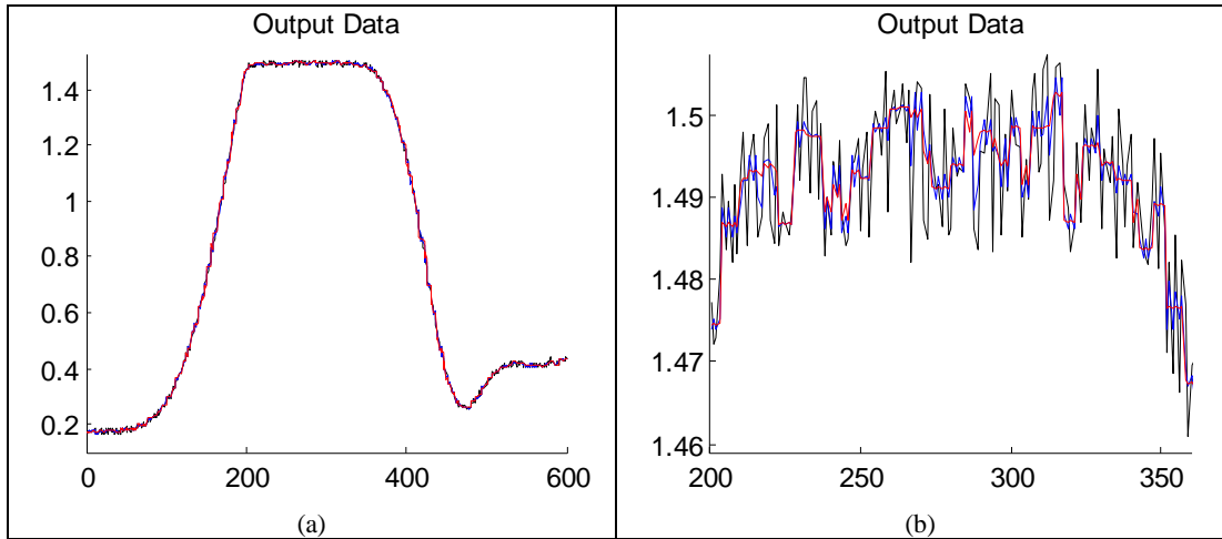
Figure 3.1.1: (Kuwahara Filtering). (a) Smoothed Displacement Data Result, (b) The samples, between 200 and 360, of Figure 3.1.1.a.
