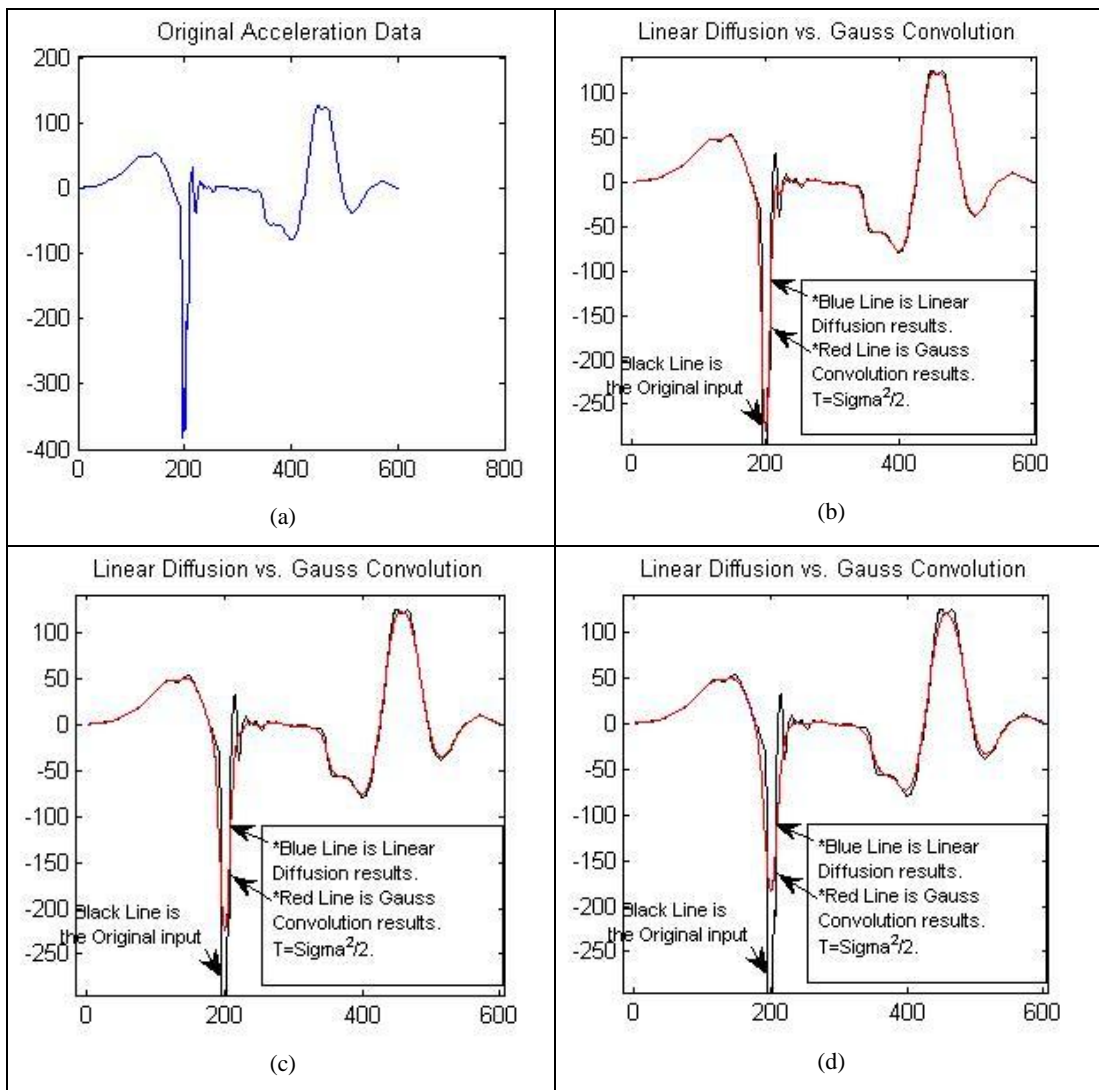
Figure 2.7.1: (Linear Diffusion Filtering vs. Gauss Convolution). T=10 , \Delta t=0.25 , (a) Original Acceleration Data, (b) Linear Diffusion for T=8 vs. Gauss Convolution for \sigma=4 , (c) Linear Diffusion for T=18 vs. Gauss Convolution for \sigma=6 , (d) Linear Diffusion for T=32 vs. Gauss Convolution for \sigma=8 .
