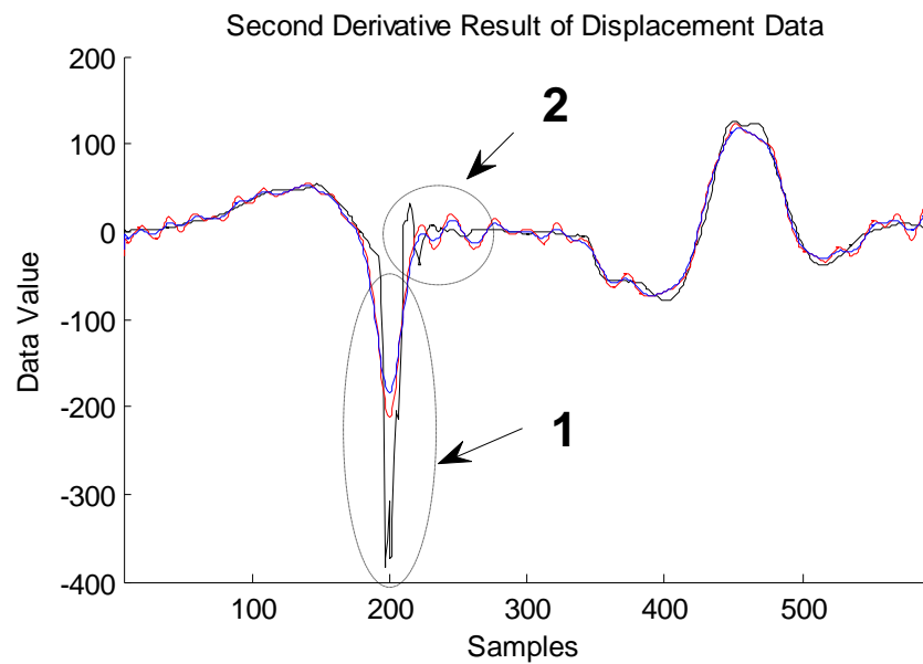
Figure 2.2.15: (Iterated Mean Filtering). The Comparative Second Derivative Results of Smoothed Displacement Data and Original Acceleration Data.
