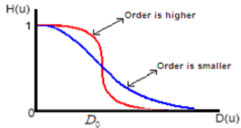
Figure 2.5.1: Butterworth Low Pass Filter Cross Section
