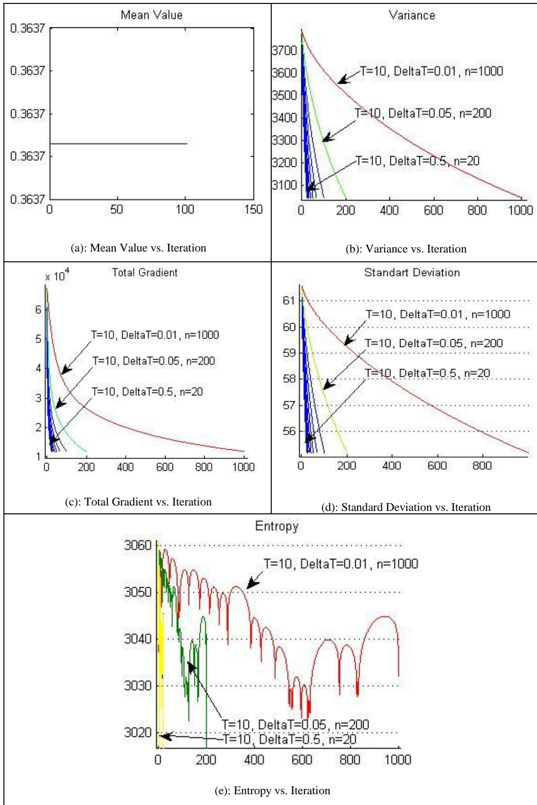
Figure 2.6.12: (Linear Diffusion Filtering). T=10, \Delta t=0.01, 0.05, 0.1, 0.15, 0.2, 0.25, 0.3, 0.35, 0.4, 0.45, 0.5 (a)Mean Value, (b)Variance, (c) Total Gradient, (d) Standard Deviation, (e) Entropy.
