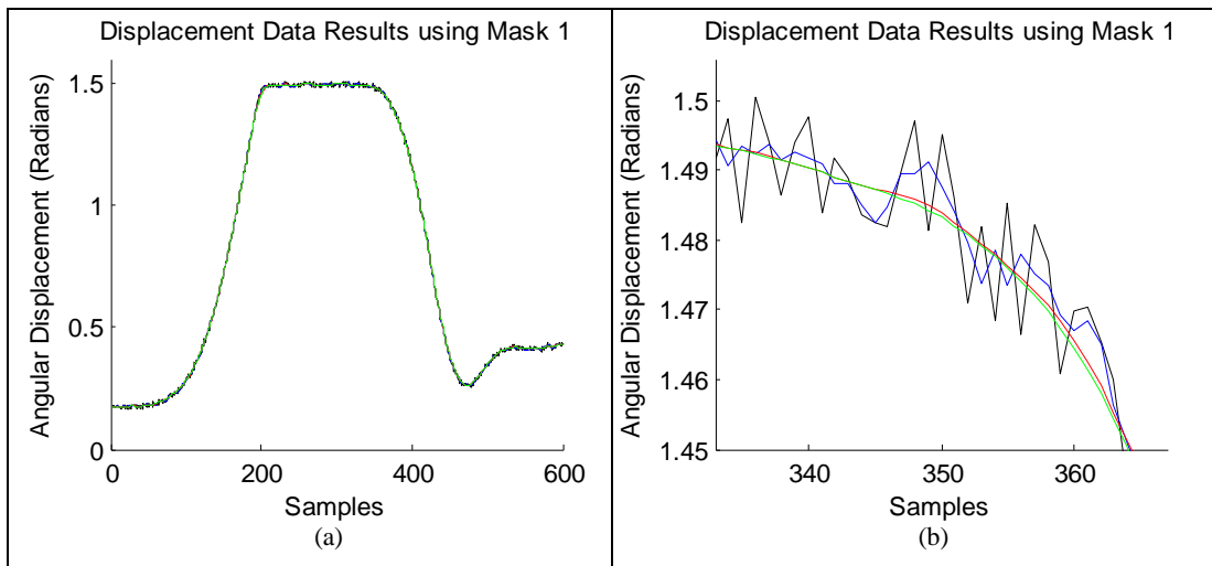
Figure 2.2.6: (Mean Filter vs. Iterated Mean Filter). (a) Displacement Data Result using the mask 1, (b) The samples, between 333 and 364, of Figure 2.2.6.a.
