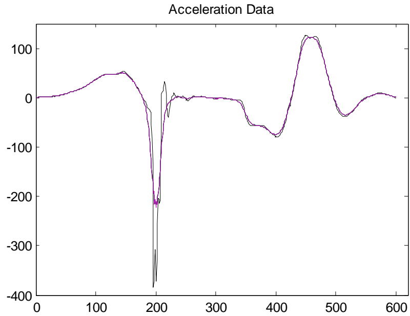
Figure 2.6.3: (Linear Diffusion Filtering). T=20 & \Delta t=0.01, 0.1, 0.2, 0.5 Black Line: The Original Data. Red Line: T=20, \Delta t=0.01, n=2000 Magenta Line: T=20, \Delta t=0.50, n=80 Blue Line: T=20, \Delta t=0.10, n=200 Green Line: T=20, \Delta t=0.20, n=100
