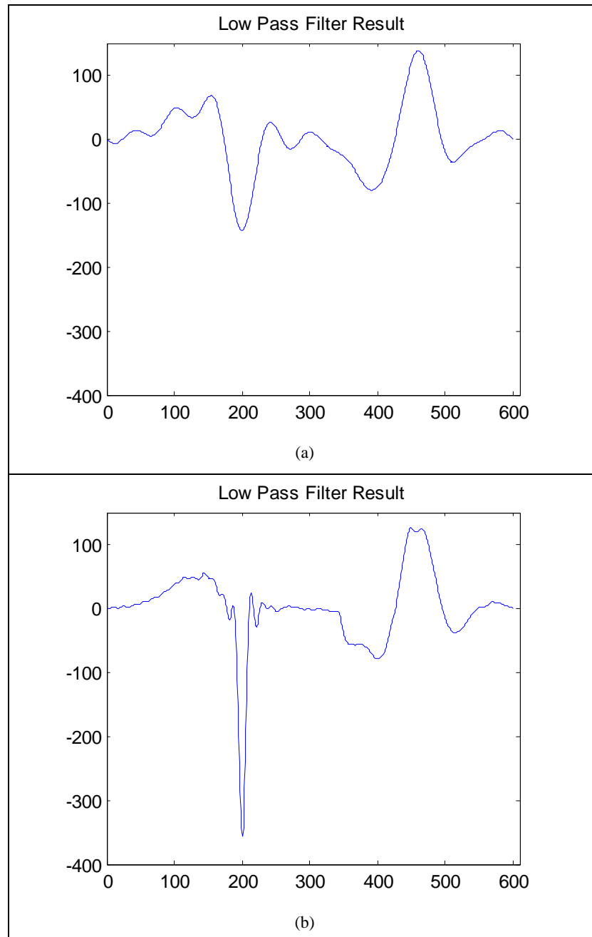
Figure 2.4.5: (Ideal Low Pass Filtering). (a) Smoothed Acceleration Data by using the Cut off Frequency=10, (b) Smoothed Acceleration Data by using the Cut off Frequency=40.
