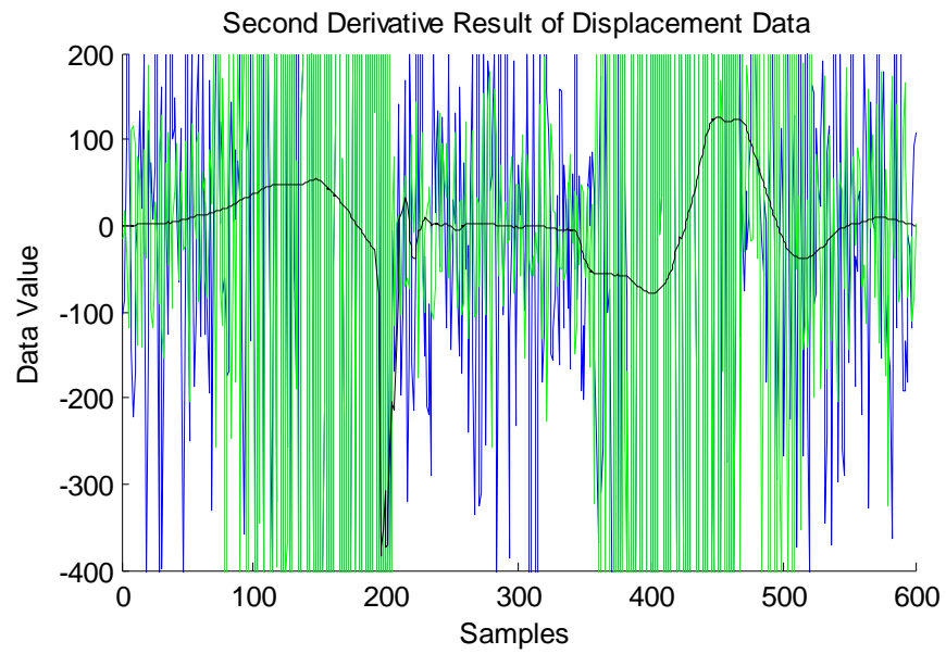
Figure 3.2.7: (Sigma Filtering). The Comparative Second Derivative Results of Smoothed Displacement Data and Original Acceleration Data.
