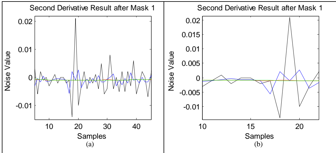
Figure 2.2.3: (Mean Filter vs. Iterated Mean Filter). (a) Second Derivative Result of Smoothed Golf Ball Data using the mask 1, (b) The samples, between 10 and 22, of Figure 2.2.3.a.
