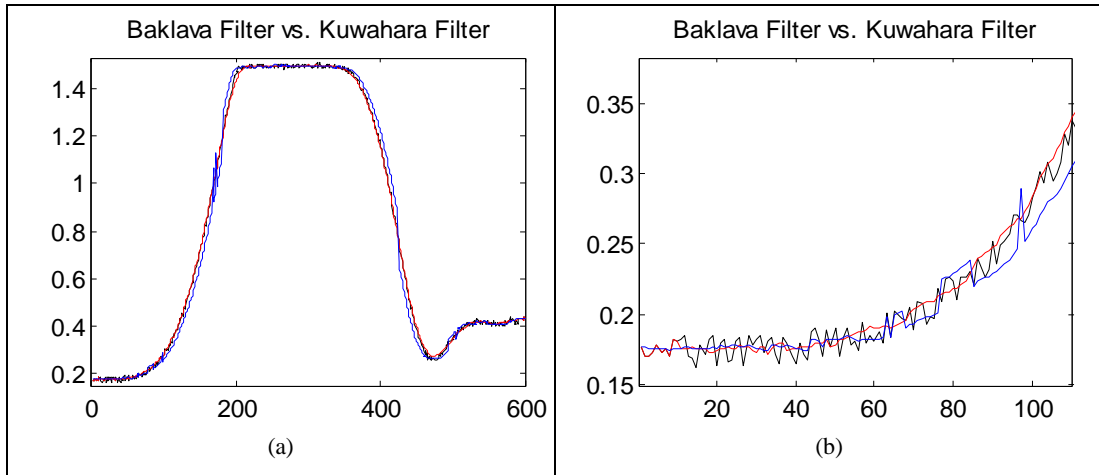
Figure 3.7.4: (Baklava Filtering vs. Kuwahara Filtering) (a) Smoothed Displacement Data Result, (b) The samples, between 0 and 110, of Figure 3.7.4.a.
