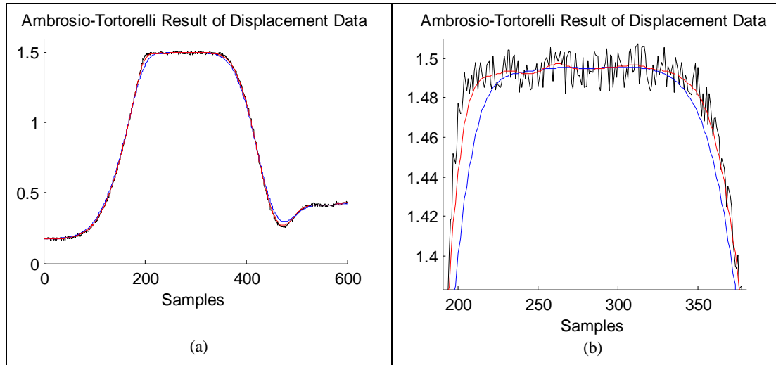
Figure 3.5.7: (Result for the Ambrosio Tortorelli Approximation of the Mumford Shah), (a) Smoothed Displacement Data Result, (b) The samples, between 190 and 380, of Figure 3.5.7.a.
