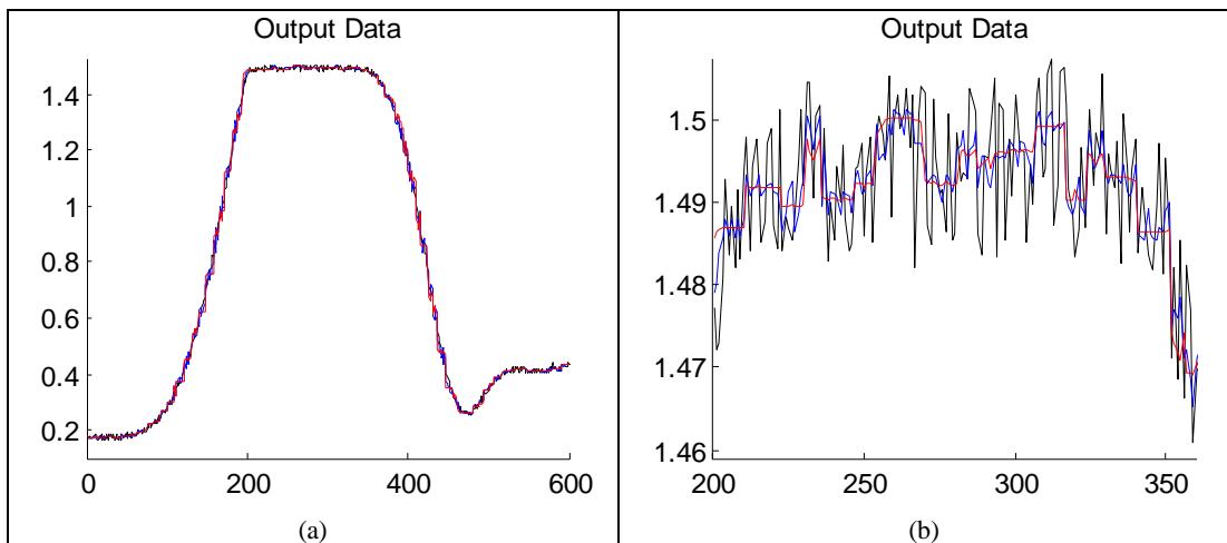
Figure 3.1.2: (Kuwahara Filtering). (a) Smoothed Displacement Data Result, (b) The samples, between 200 and 360, of Figure 3.1.2.a.
