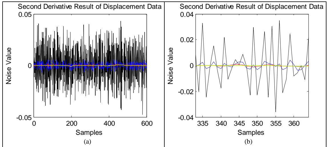
Figure 2.3.4: (Gaussian Filtering). (a) Second Derivative Result of Smoothed Displacement Data for \sigma=1, 2, 4, 6 , \text{size}=6*\sigma+1 , (b) The samples, between 333 and 364, of Figure 2.3.4.a.
