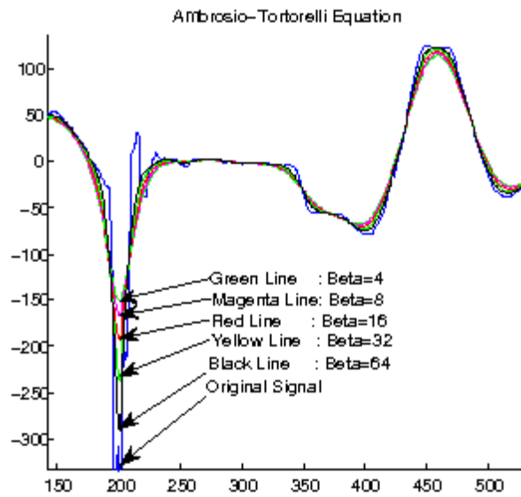
Figure 3.5.5: (Result for the Ambrosio Tortorelli Approximation of the Mumford Shah)
