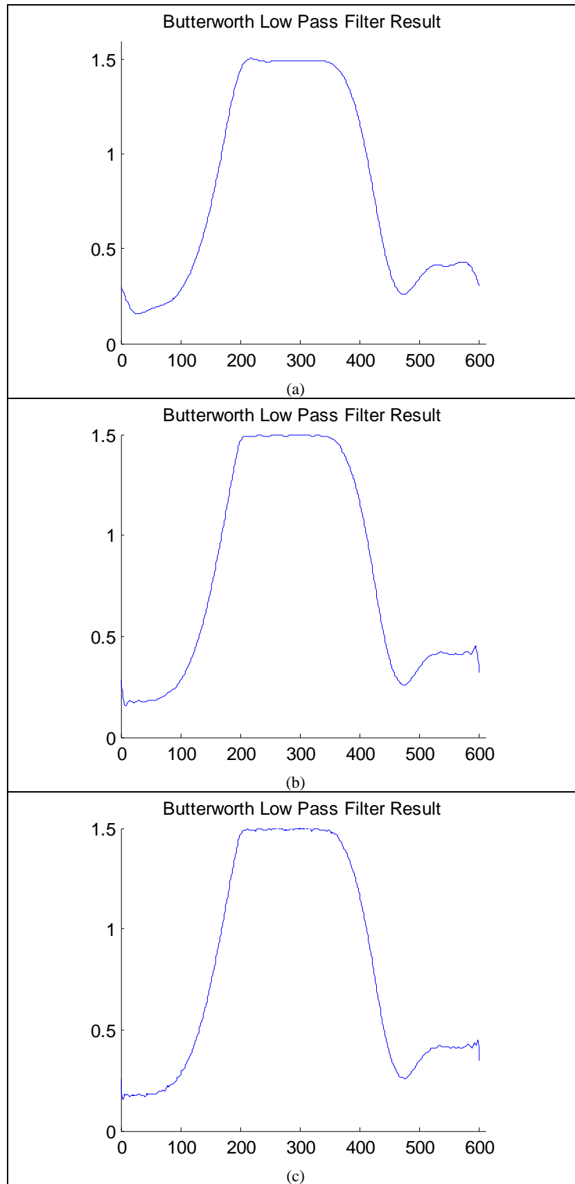
Figure 2.5.2: (Butterworth Low Pass Filtering). (a) Smoothed Displacement Data by using the Cut off Frequency=10 and Order=3, (b) Smoothed Displacement Data by using the Cut off Frequency=40 and Order=3, (c) Smoothed Displacement Data by using the Cut off Frequency=100 and Order=3.
