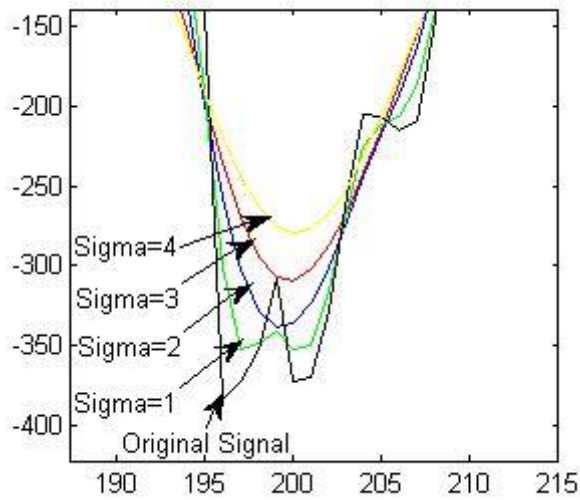
Figure 2.3.7: (Gaussian Filtering). Results between 186 and 215 for \sigma=1, 2, 3, 4 , \text{size}=6*\sigma+1 .
