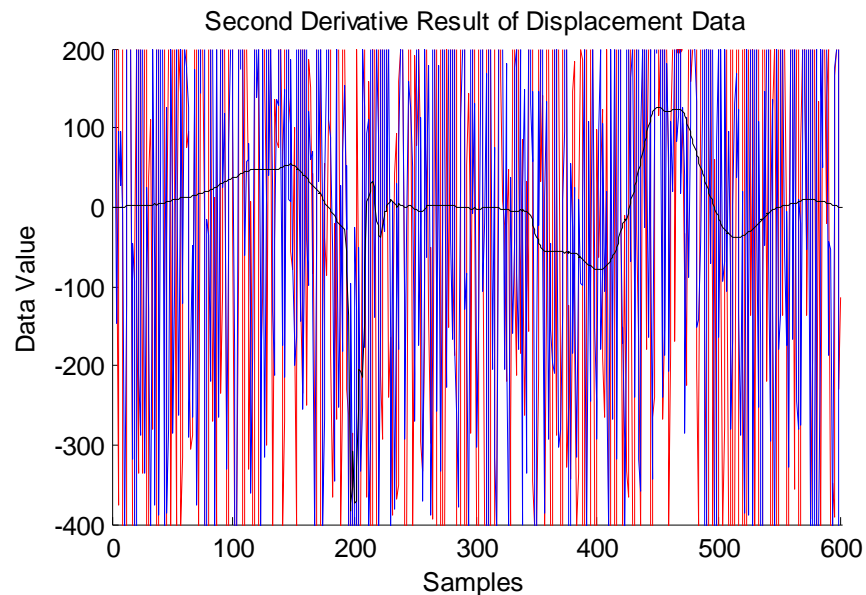
Figure 2.2.13: (Mean Filtering). The Comparative Second Derivative Results of Smoothed Displacement Data and Original Acceleration Data.
