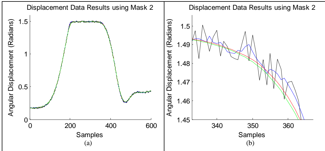
Figure 2.2.7: (Mean Filter vs. Iterated Mean Filter). (a) Displacement Data Result using the mask 2, (b) The samples, between 333 and 364, of Figure 2.2.7.a.
