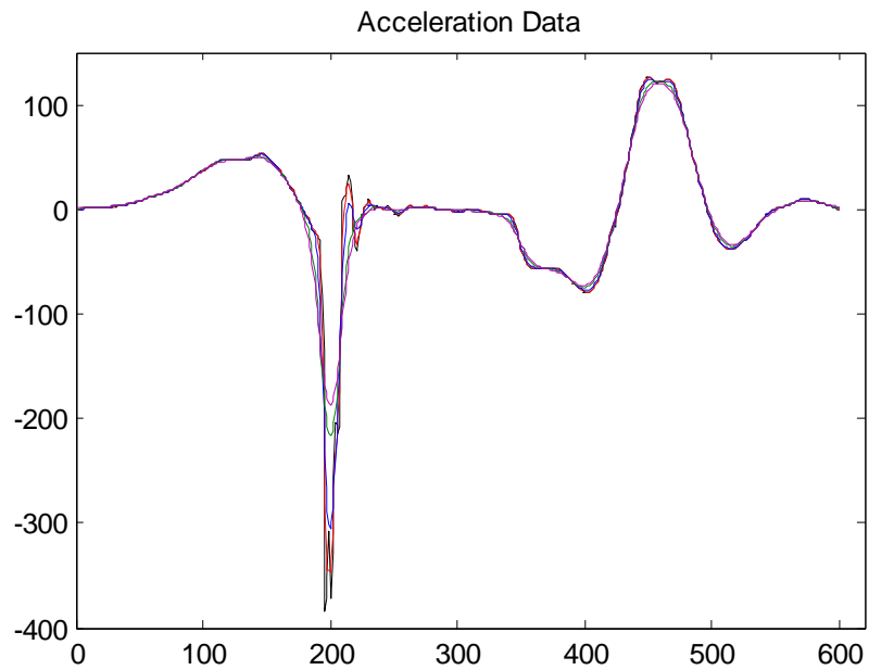
Figure 2.6.4: (Linear Diffusion Filtering). \Delta t=0.1 & T=1, 5, 20, 30 Black Line: The Original Data. Red Line: T=1, \Delta t=0.1, n=10 Magenta Line: T=30, \Delta t=0.1, n=300 Blue Line: T=5, \Delta t=0.1, n=50 Green Line: T=20, \Delta t=0.1, n=200
