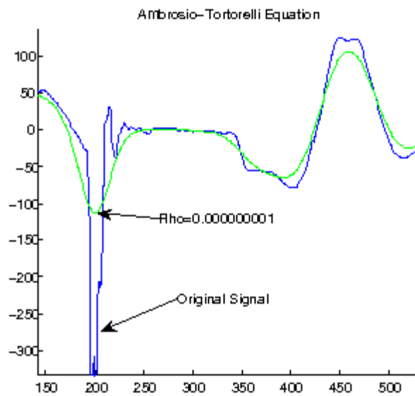
Figure 3.5.6: (Result for the Ambrosio Tortorelli Approximation of the Mumford Shah)
