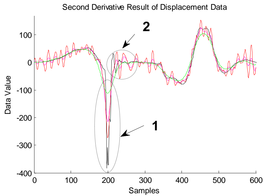
Figure 2.6.14: (Linear Diffusion Filtering). The Comparative Second Derivative Results of Smoothed Displacement Data and Original Acceleration Data.
