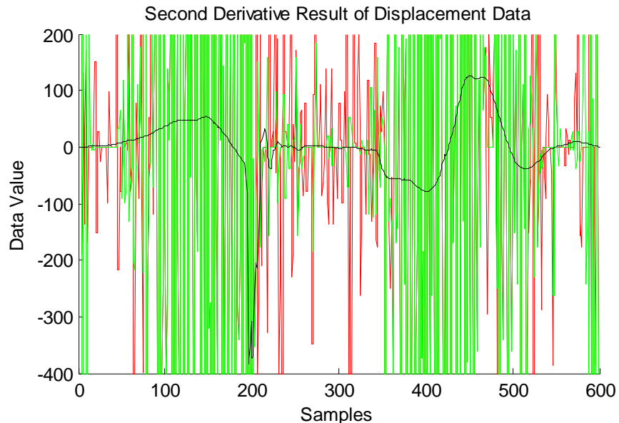
Figure 3.3.8: (Iterative Median Filtering). The Comparative Second Derivative Results of Smoothed Displacement Data and Original Acceleration Data. Black Line is the Original Acceleration Data.
