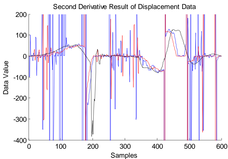
Figure 3.1.8: (Iterative Kuwahara Filtering). The Comparative Second Derivative Results of Smoothed Displacement Data and Original Acceleration Data. Black Line is the Original Acceleration Data. Blue Line : Second Derivative of Smoothed Displacement Data by using the Mask Size=41 for 3 iteration Red Line : Second Derivative of Smoothed Displacement Data by using the Mask Size=61 for 3 iteration
