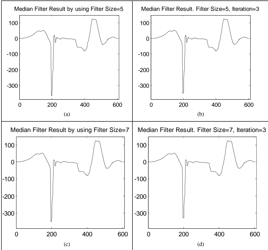
Figure 3.3.3: (Median Filtering). (a) Filter Size=5, (b) Filter Size=5 & Iteration number=3, (c) Filter Size=7, (d) Filter Size=7 & Iteration number=3.
