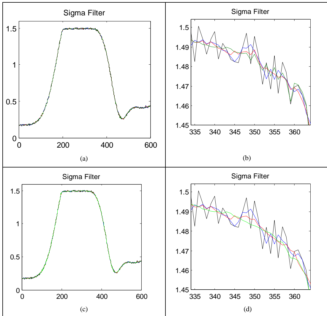
Figure 3.2.3: (Sigma Filtering), Sigma is constant.
