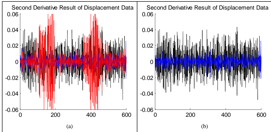
Figure 3.7.9: (Baklava Filtering vs. Kuwahara Filtering). (a) Second Derivative Result of Smoothed Displacement Data using Baklava Filtering & Kuwahara Filtering for the Mask Size=7 (b) Same as Figure 3.7.9.a except Kuwahara Filtering Result .
