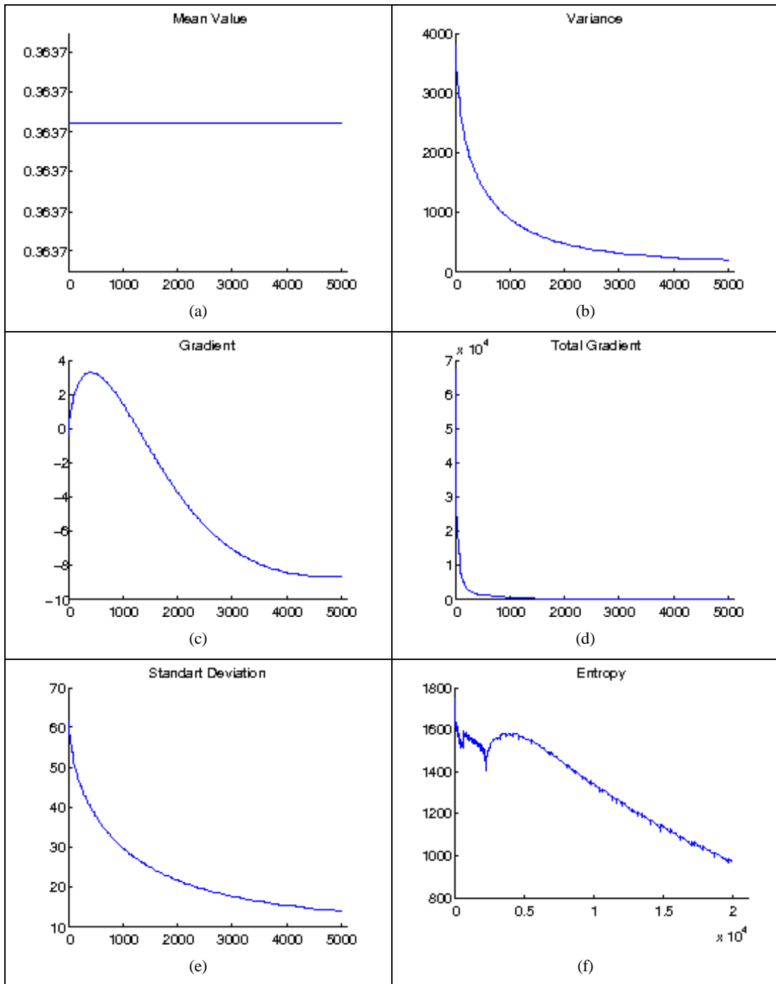
Figure 3.6.3: (Results for the Ambrosio Tortorelli Approximation of the Mumford Shah)
