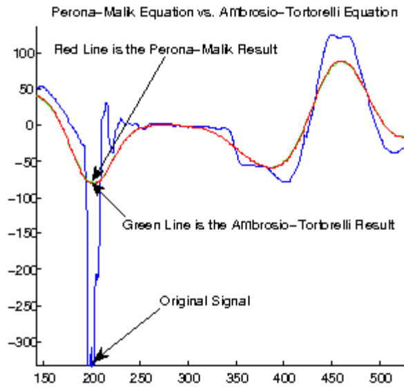
Figure 3.6.1: (Perona-Malik Equation vs. Ambrosio-Tortorelli Equation) Green Line : Ambrosio-Tortorelli Result for T=200 , \Delta t=0.4 , \alpha=8 , \beta=0.05 , \rho=0.000000001 Red Line : Perona-Malik Result for T=200 , \Delta t=0.4 , \lambda=10 , and \sigma=18 .
