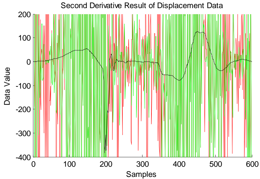
Figure 3.3.7: (Median Filtering). The Comparative Second Derivative Results of Smoothed Displacement Data and Original Acceleration Data. Black Line is the Original Acceleration Data.
