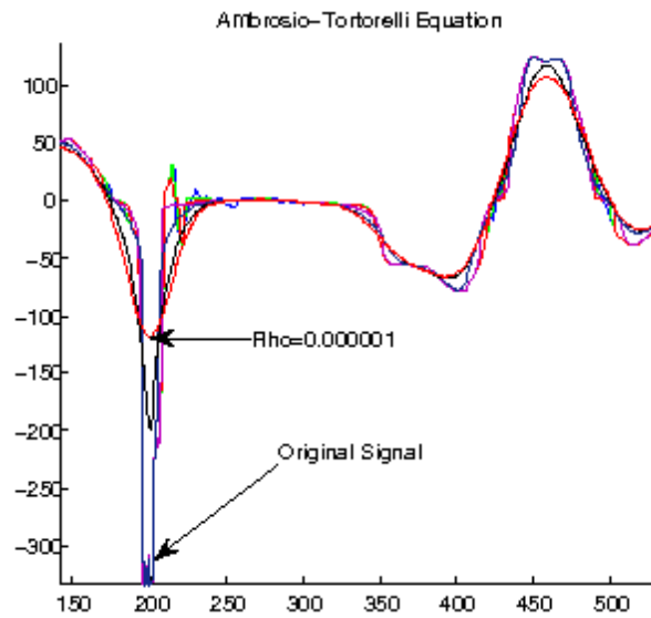
Figure 3.5.2: (Result for the Ambrosio Tortorelli Approximation of the Mumford Shah) The results for T=100 , \Delta t=0.4 , \alpha=2 , \beta=0.025 , \rho=0.05, 0.01, 0.001, 0.0001, 0.00001, 0.000001
