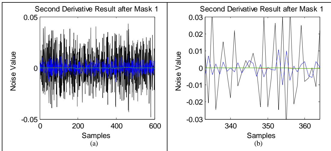
Figure 2.2.8: (Mean Filter vs. Iterated Mean Filter). (a) Second Derivative Result of Smoothed Displacement Data using the mask 1, (b) The samples, between 333 and 364, of Figure 2.2.8.a.
