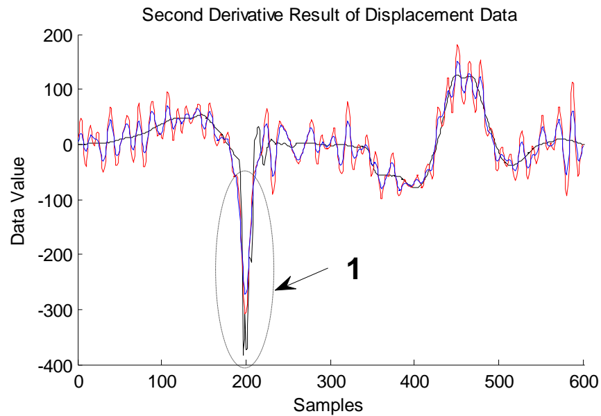
Figure 2.2.14: (Iterated Mean Filtering). The Comparative Second Derivative Results of Smoothed Displacement Data and Original Acceleration Data.
