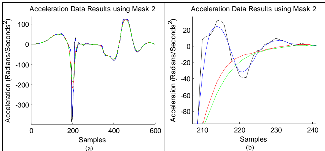
Figure 2.2.12: (Mean Filter vs. Iterated Mean Filter). (a) Acceleration Data Result using the mask 2, (b) The samples, between 207 and 242, of Figure 2.2.12.a.
