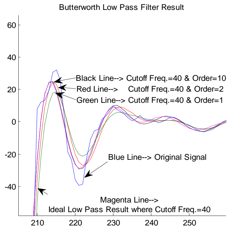
Figure 2.5.5: (Butterworth Low Pass Filtering). Zoom in Smoothed Acceleration Data by using Cut off Frequency=40 and Order=1,2 and 10.
