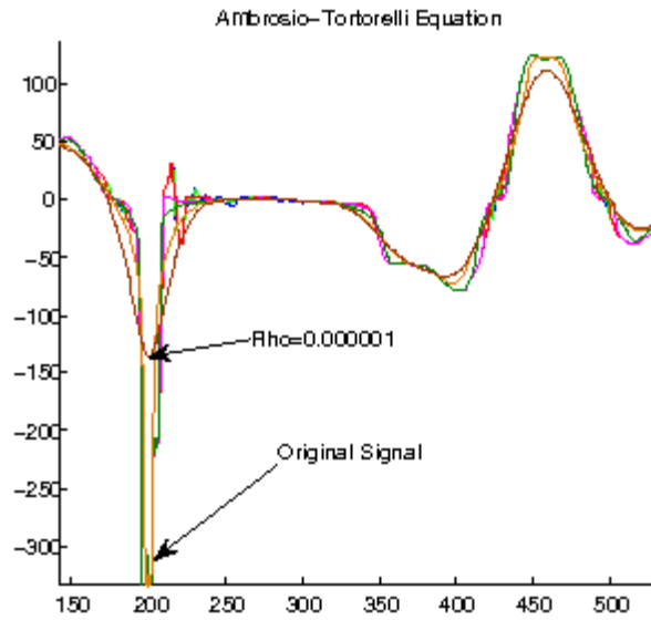
Figure 3.5.1: (Result for the Ambrosio Tortorelli Approximation of the Mumford Shah) The results for T=100 , \Delta t=0.4 , \alpha=8 , \beta=0.1 , \rho=0.05, 0.01, 0.001, 0.0001, 0.00001, 0.000001
