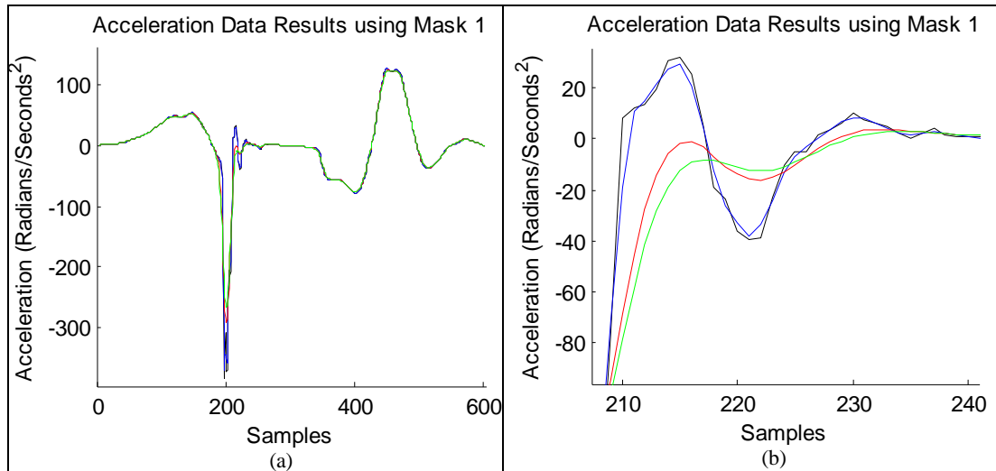
Figure 2.2.11: (Mean Filter vs. Iterated Mean Filter). (a) Acceleration Data Result using the mask 1, (b) The samples, between 207 and 242, of Figure 2.2.11.a.
