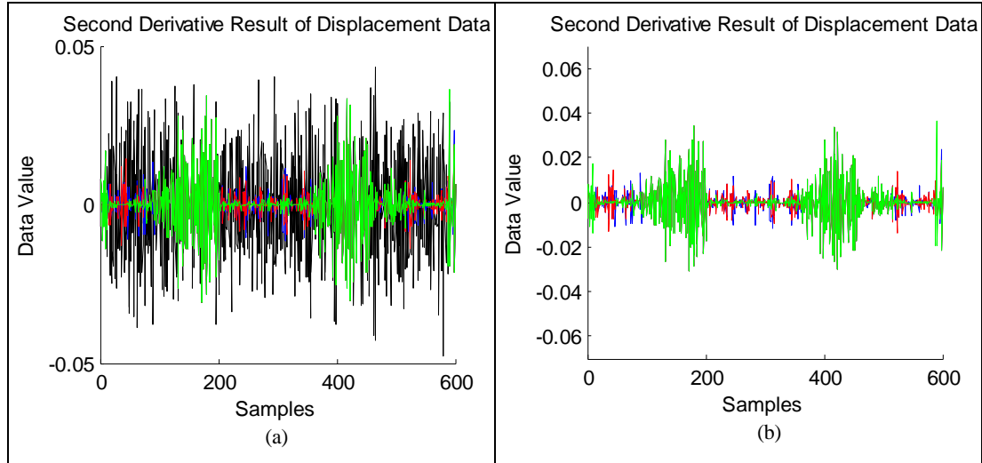
Figure 3.3.5: (Median Filtering). (a) Second Derivative Result of Smoothed Displacement Data using Filter Size = 5, 7, 21 (b) Same as Figure 3.3.5.a except Original Displacement Data (Black Line) .
