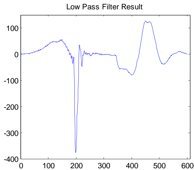
Figure 2.4.6: (Ideal Low Pass Filtering). Smoothed Acceleration Data by using the Cut off Frequency=100.
