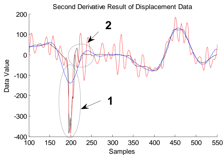
Figure 2.5.8: (Butterworth Low Pass Filtering). The Comparative Second Derivative Results of Smoothed Displacement Data and Original Acceleration Data.
