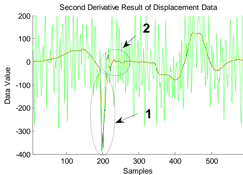
Figure 2.3.9: (Gaussian Filtering). The Comparative Second Derivative Results of Smoothed Displacement Data and Original Acceleration Data.
