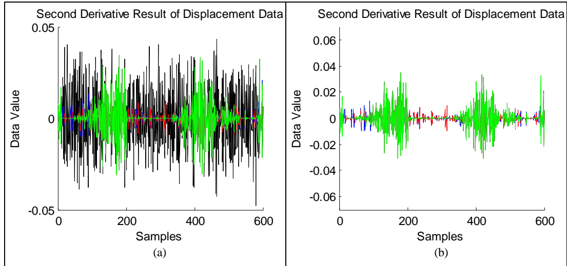
Figure 3.3.6: (Median Filtering). (a) Second Derivative Result of Smoothed Displacement Data using Filter Size = 5, 7, 21 for 3 iteration (b) Same as Figure 3.3.6.a except Original Displacement Data (Black Line) .
