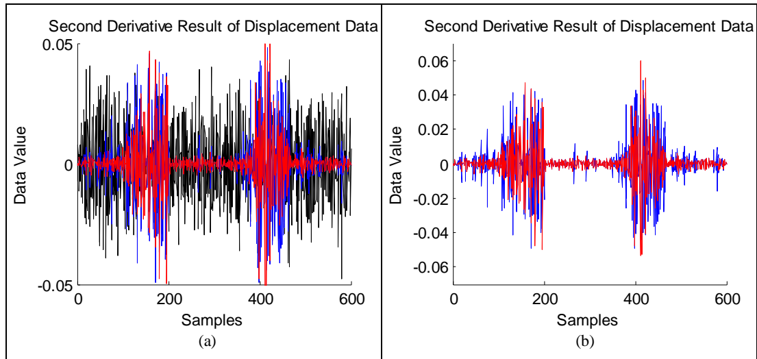
Figure 3.2.6: (Sigma Filtering). (a) Second Derivative Result of Smoothed Displacement Data using \sigma=0.015, 0.01 and Mask Size = 7 (b) Same as Figure 3.2.6.a except Original Displacement Data (Black Line).
