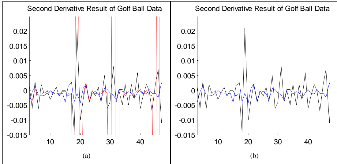
Figure 3.7.8: (Baklava Filtering vs. Kuwahara Filtering). (a) Second Derivative Result of Smoothed Golf Ball Data using Baklava Filtering & Kuwahara Filtering for the Mask Size=7 (b) Same as Figure 3.7.8.a except Kuwahara Filtering Result .
