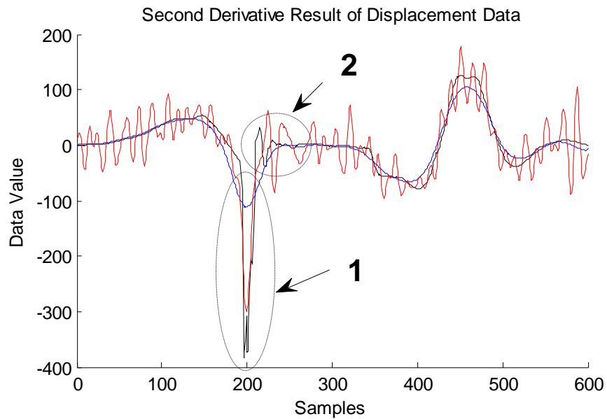
Figure 3.5.10: (Ambrosio Tortorelli Approximation of the Mumford Shah). The Comparative Second Derivative Results of Smoothed Displacement Data and Original Acceleration Data.
