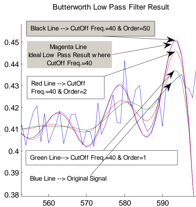
Figure 2.5.3: (Butterworth Low Pass Filtering). Blue Line is the Original input data. Green Line, Red Line and Black Line are the Smoothed Displacement Data by using the Cut off Frequency is 40 and Orders are 1, 2 and 50. Magenta Line is the Ideal Low Pass Filter Result where Cut off Frequency=40.
