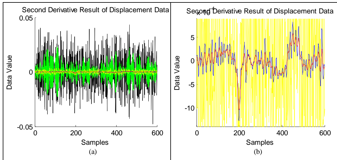
Figure 2.6.13: (Linear Diffusion Filtering). (a) Second Derivative Result of Smoothed Displacement Data (b) Same as Figure 2.6.13.a except Original Displacement Data (Black Line) and Green Line.
