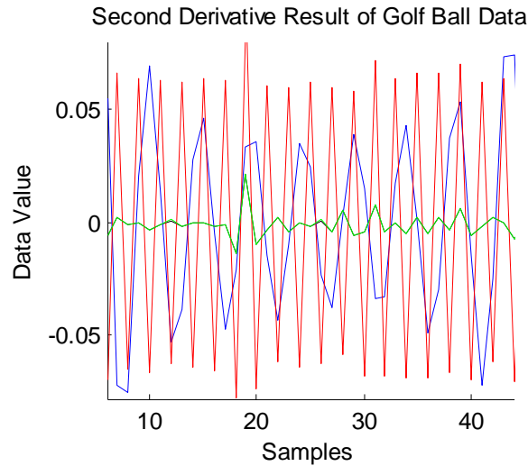
Figure 2.4.7: (Ideal Low Pass Filtering). Second Derivative Result of Smoothed Golf Ball Data using Cut off Frequency=10, 24 and 25.
