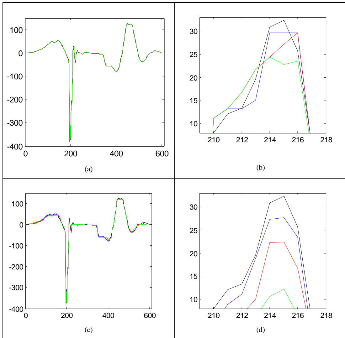
Figure 3.2.4: (Sigma Filtering), Mask Size is constant.
