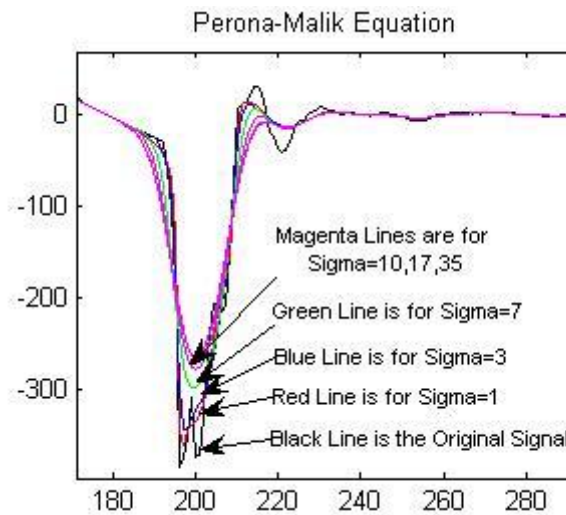
Figure 3.4.4: (Perona Malik Filtering). Results between the samples of 176 and 284 for \lambda=10 , T=10 , \Delta t=0.25 and various \sigma=1, 3, 7, 10, 17, 35 .
