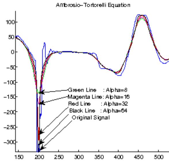
Figure 3.5.4: (Result for the Ambrosio Tortorelli Approximation of the Mumford Shah) The results for T=100 , \Delta t=0.4 , \alpha=8, 16, 32, 64 , \beta=0.025 , \rho=0.000001 .
