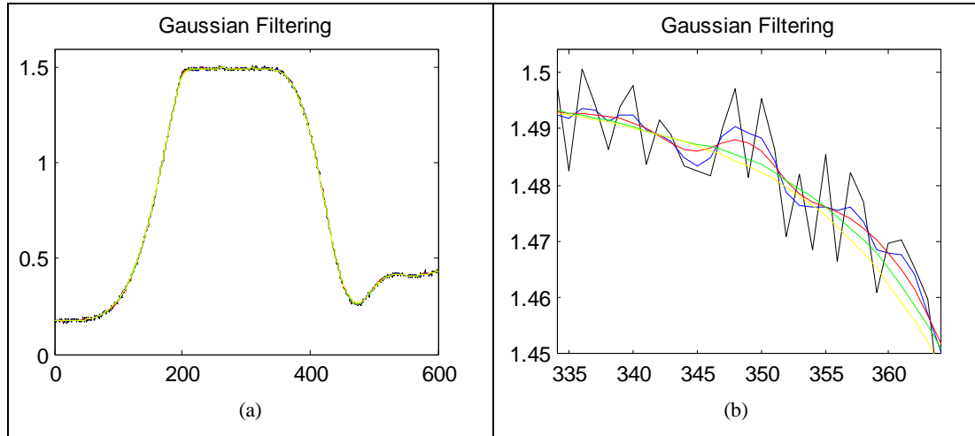
Figure 2.3.2: (Gaussian Filtering). (a) Displacement Data Results for \sigma=1, 2, 4, 6 , \text{size}=6*\sigma+1 , (b) The samples, between 333 and 364, of Figure 2.3.2.a.
