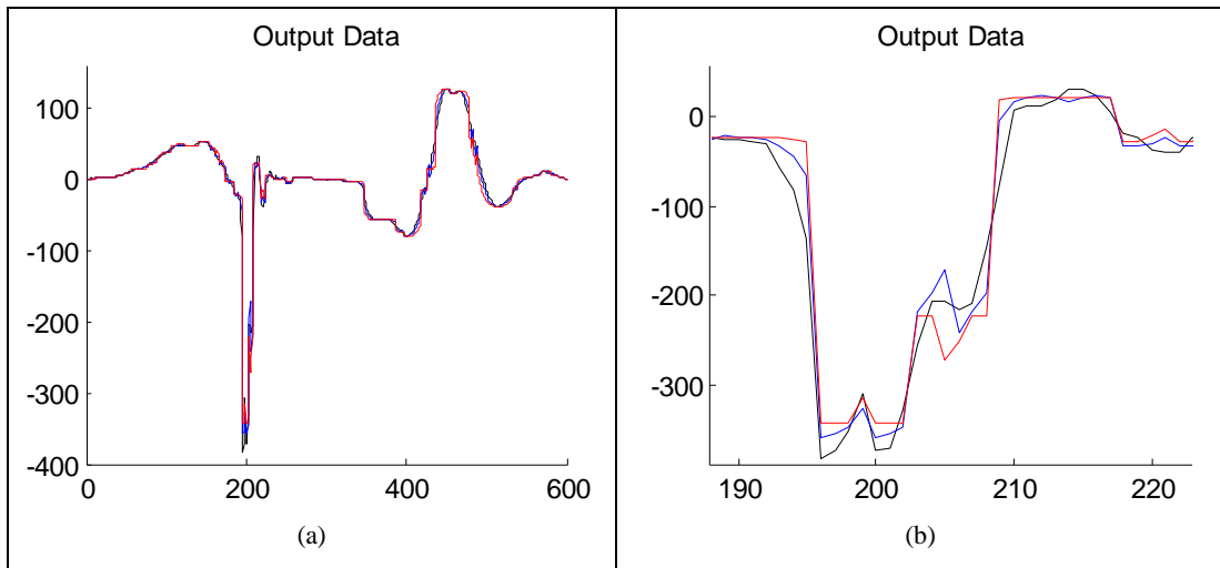
Figure 3.1.4: (Kuwahara Filtering). (a) Smoothed Acceleration Data Result, (b) The samples, between 190 and 220, of Figure 3.1.4.a.
