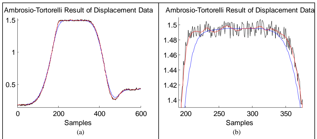
Figure 3.5.8: (Result for the Ambrosio Tortorelli Approximation of the Mumford Shah), (a) Smoothed Displacement Data Result, (b) The samples, between 190 and 380, of Figure 3.5.8.a.
