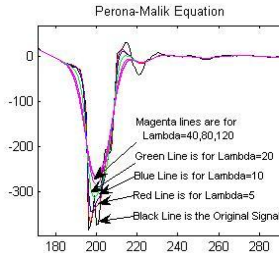
Figure 3.4.5: (Perona Malik Filtering). Results between the samples of 176 and 284 for \sigma=3 , T=10 , \Delta t=0.25 and various \lambda=5, 10, 20, 40, 80, 120 .
