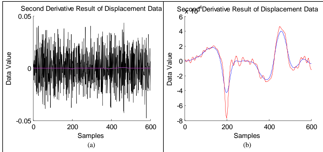
Figure 3.5.9: (Ambrosio Tortorelli Approximation of the Mumford Shah). (a) Second Derivative Result of Smoothed Displacement Data (b) Same as Figure 3.5.9.a except Original Displacement Data (Black Line).
