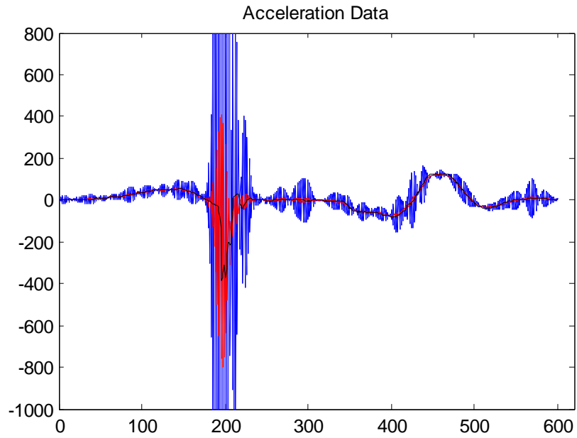
Figure 2.6.7: (Linear Diffusion Filtering). T=20 & \Delta t=0.53, 0.55
