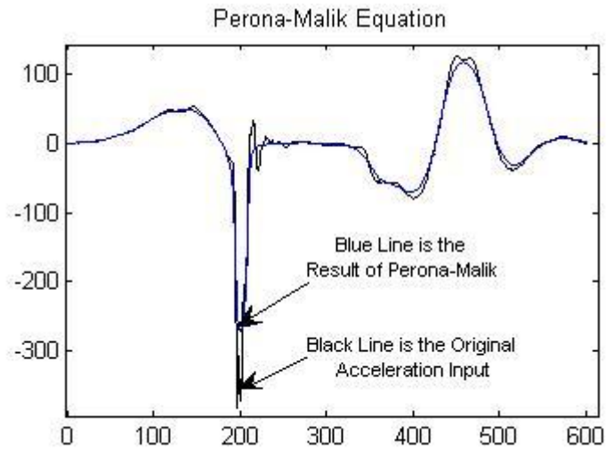
Figure 3.4.6: (Perona Malik Filtering). ) Smoothed Acceleration Data by using \sigma=3 , \lambda=10 , T=50 and \Delta t=0.05 .
