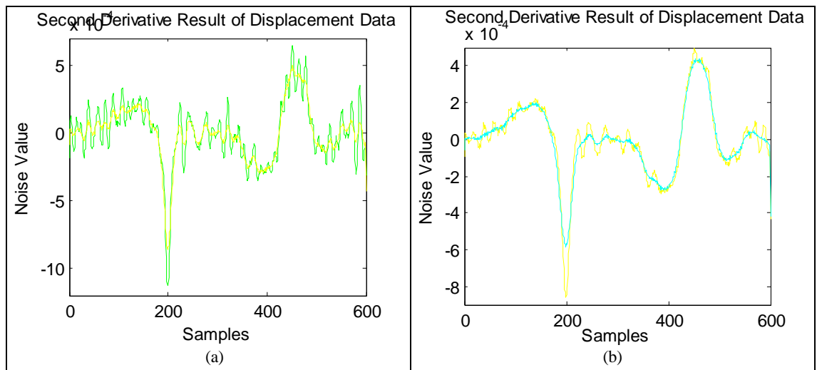
Figure 2.3.5: (Gaussian Filtering). (a) Second Derivative Result of Smoothed Displacement Data for \sigma=4, 6 , \text{size}=6*\sigma+1 , (b) Second Derivative Result of Smoothed Displacement Data for \sigma=6, 10 , \text{size}=6*\sigma+1 ,
