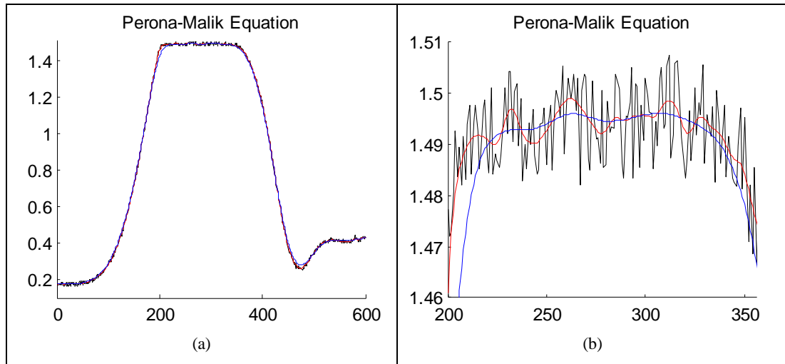
Figure 3.4.1: (Perona Malik Filtering), (a) Smoothed Displacement Data Result, (b) The samples, between 200 and 360, of Figure 3.4.1.a.
