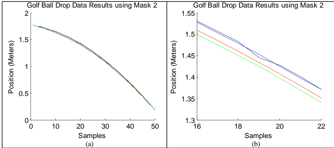
Figure 2.2.2: (Mean Filter vs. Iterated Mean Filter). (a) Golf Ball Data Result using the mask 2, (b) The samples, between 16 and 22, of Figure 2.2.2.a.
