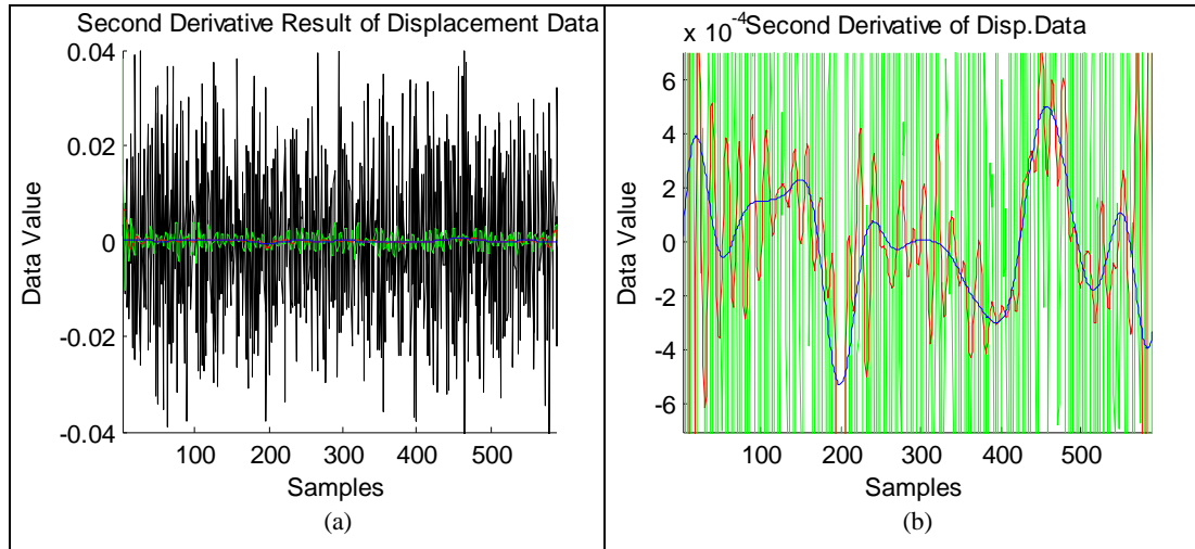
Figure 2.5.6: (Butterworth Low Pass Filtering). (a) Second Derivative Result of Smoothed Displacement Data using Cut off Frequency=10, 40, 100, and Order=3 (b) Same as Figure 2.5.6.a except Original Displacement Data (Black Line).
