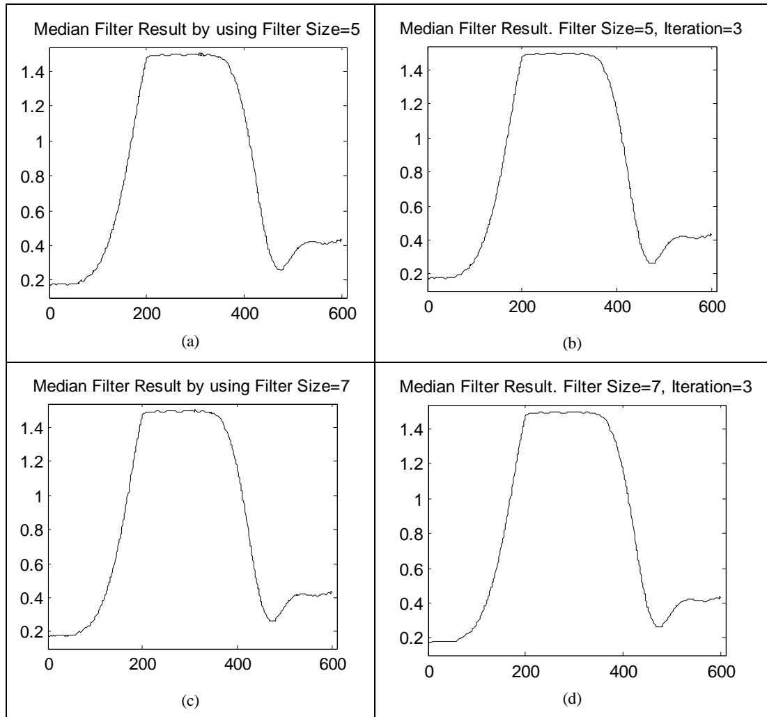
Figure 3.3.2: (Median Filtering). (a) Filter Size=5, (b) Filter Size=5 & Iteration number=3, (c) Filter Size=7, (d) Filter Size=7 & Iteration number=3.
