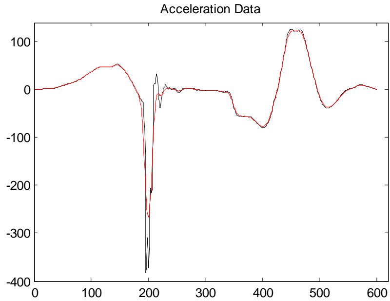
Figure 2.6.10: (Linear Diffusion Filtering). T=10, \Delta t=0.1
