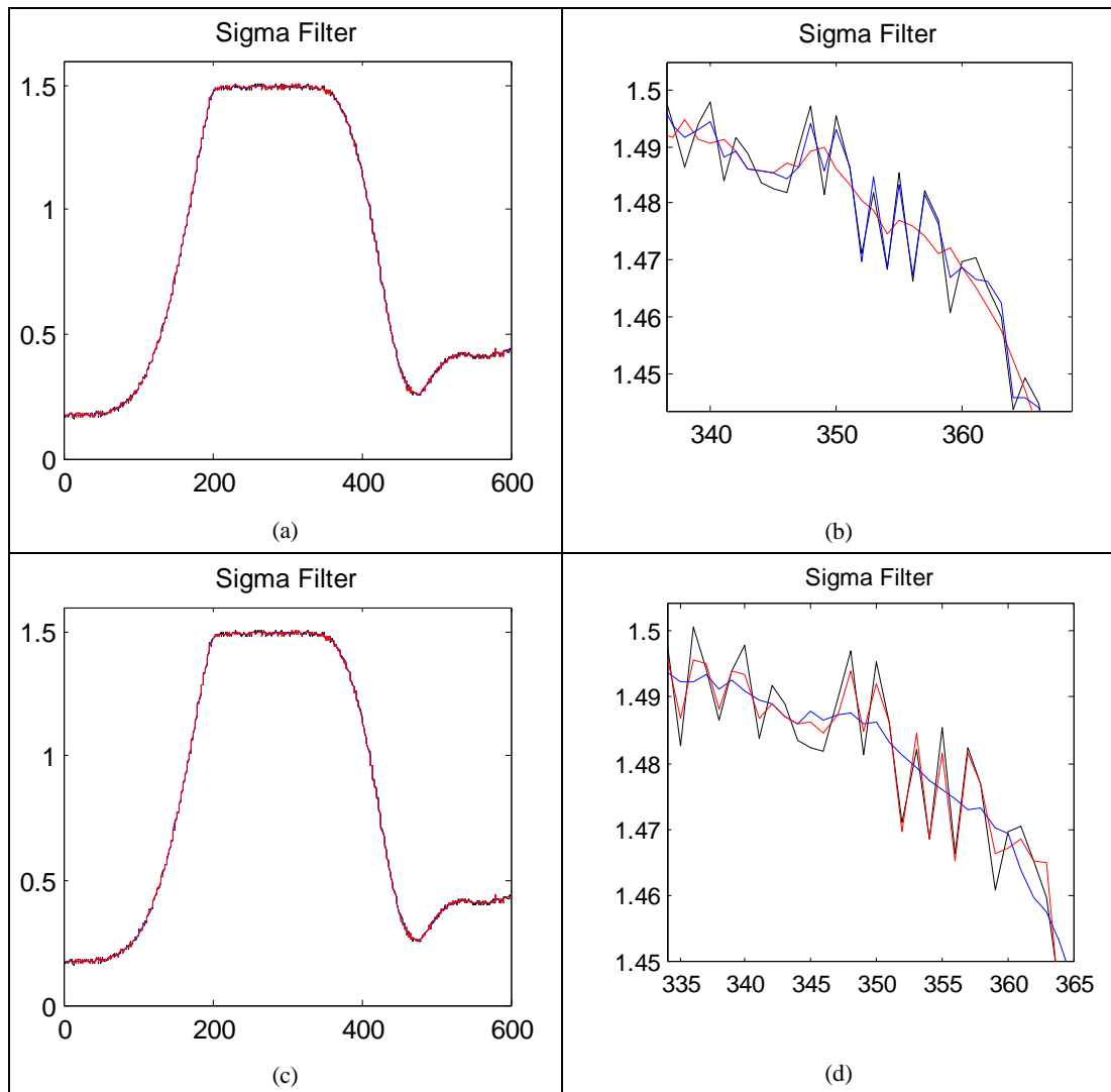
Figure 3.2.2: (Sigma Filtering), Mask Size is constant.
