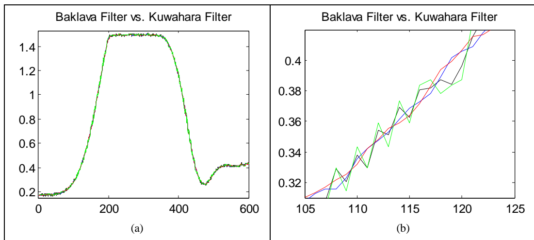
Figure 3.7.3: (Baklava Filtering vs. Kuwahara Filtering) (a) Smoothed Displacement Data Result, (b) The samples, between 105 and 125, of Figure 3.7.3.a.
