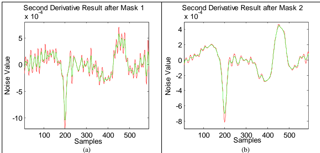
Figure 2.2.10: (Iterated Mean Filter). (a) Second Derivative Result of Smoothed Displacement Data using the mask 1 (1x3), (b) Second Derivative Result of Smoothed Displacement Data using the mask 2 (1x5).
