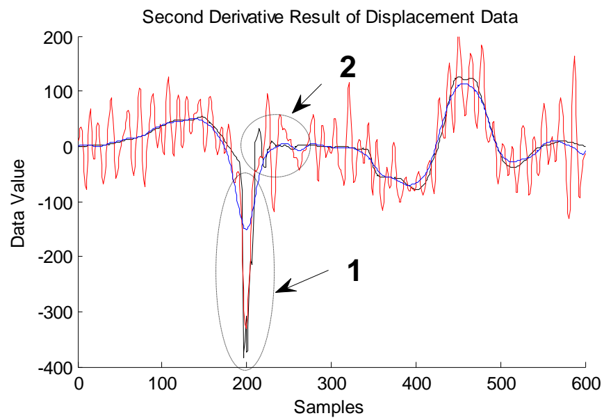
Figure 3.4.9: (Perona Malik Filtering). The Comparative Second Derivative Results of Smoothed Displacement Data and Original Acceleration Data.
