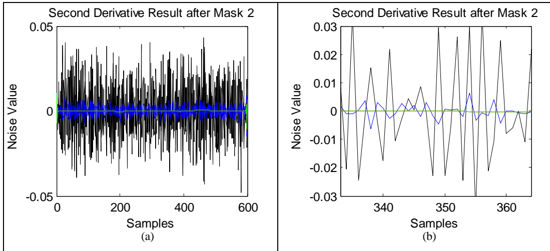
Figure 2.2.9: (Mean Filter vs. Iterated Mean Filter). (a) Second Derivative Result of Smoothed Displacement Data using the mask 2, (b) The samples, between 333 and 364, of Figure 2.2.9.a.
