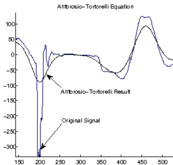
Figure 3.6.2: (Result for the Ambrosio Tortorelli Approximation of the Mumford Shah) The result for Result: T=200 , \Delta t=0.4 , \alpha=8 , \beta=0.05 , \rho=0.000001
