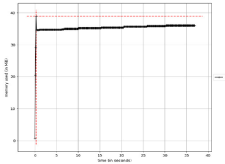
Figure 2 Memory overhead
