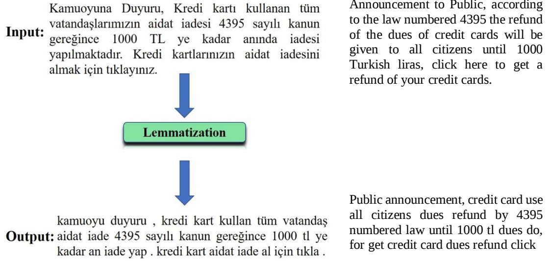
Figure 11 Lemmatization Example
