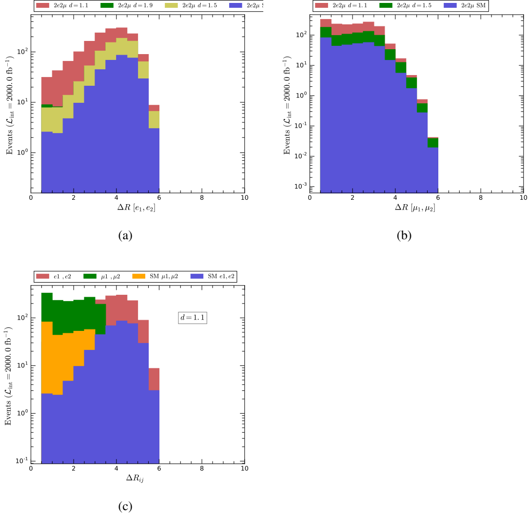
Figure 4.23: Various distributions of the process e^+e^- \rightarrow 2e2\mu in the framework of unparticle stuff with \sqrt{s} = 3 TeV at CLIC
