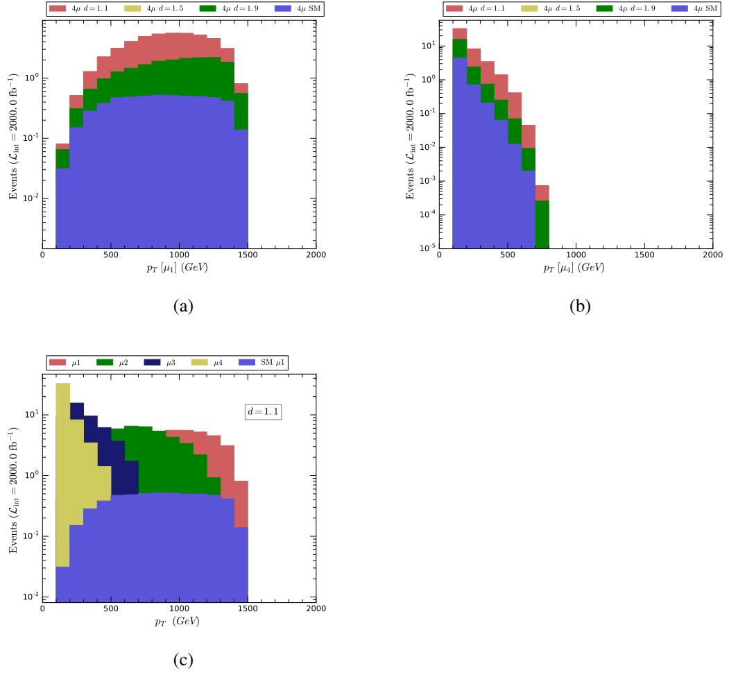
Figure 4.22: Various distributions of the process e^+e^- \rightarrow 4\mu in the framework of unparticle stuff with \sqrt{s} = 3 \text{ TeV} at CLIC
