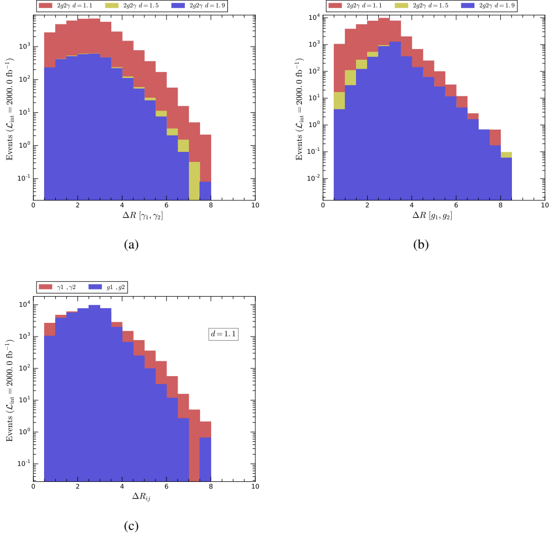
Figure 4.8: Various distributions of the process e^+e^- \rightarrow 2\gamma 2g in the framework of unparticle stuff with \sqrt{s} = 3 TeV at CLIC
