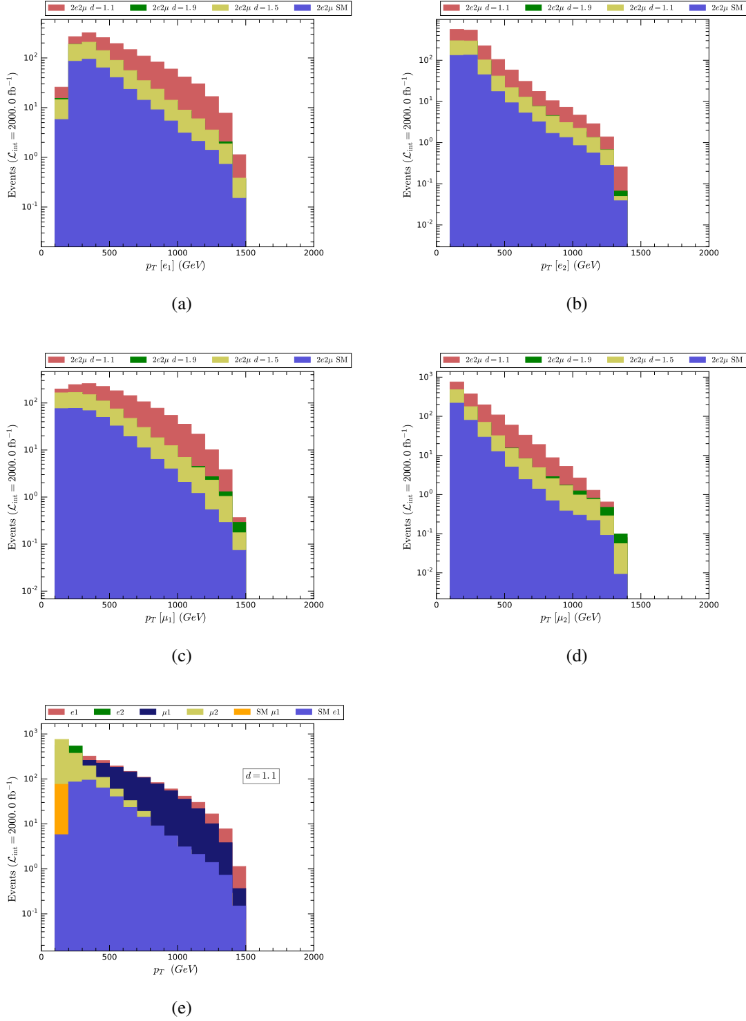
Figure 4.25: Various distributions of the process e^+e^- \rightarrow 2e2\mu in the framework of unparticle stuff with \sqrt{s} = 3 TeV at CLIC
