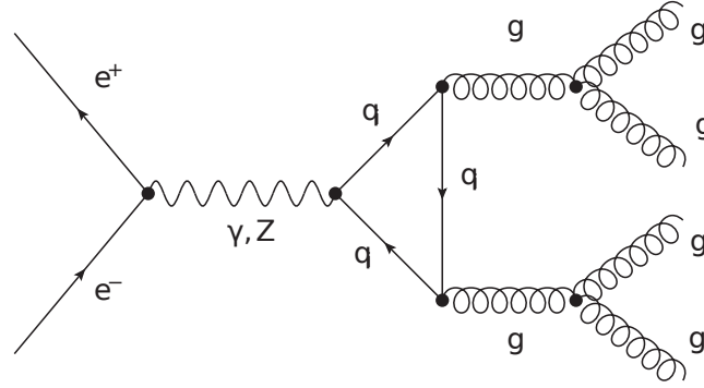
Figure 4.5: A sample diagram contributing e^+e^- \rightarrow 4g at one-loop in the SM.
