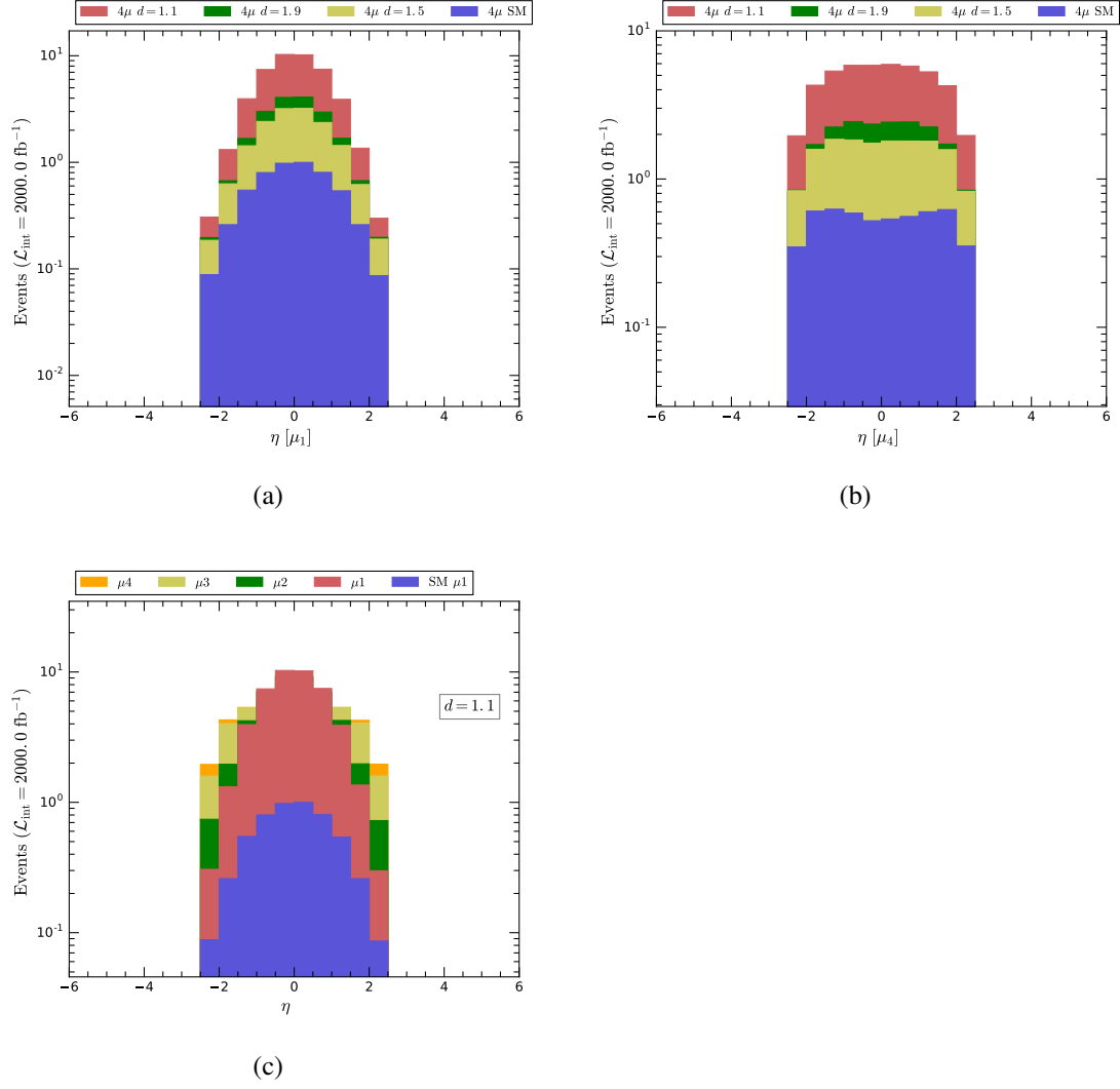
Figure 4.21: Various distributions of the process e^+e^- \rightarrow 4\mu in the framework of unparticle stuff with \sqrt{s} = 3 \text{ TeV} at CLIC
