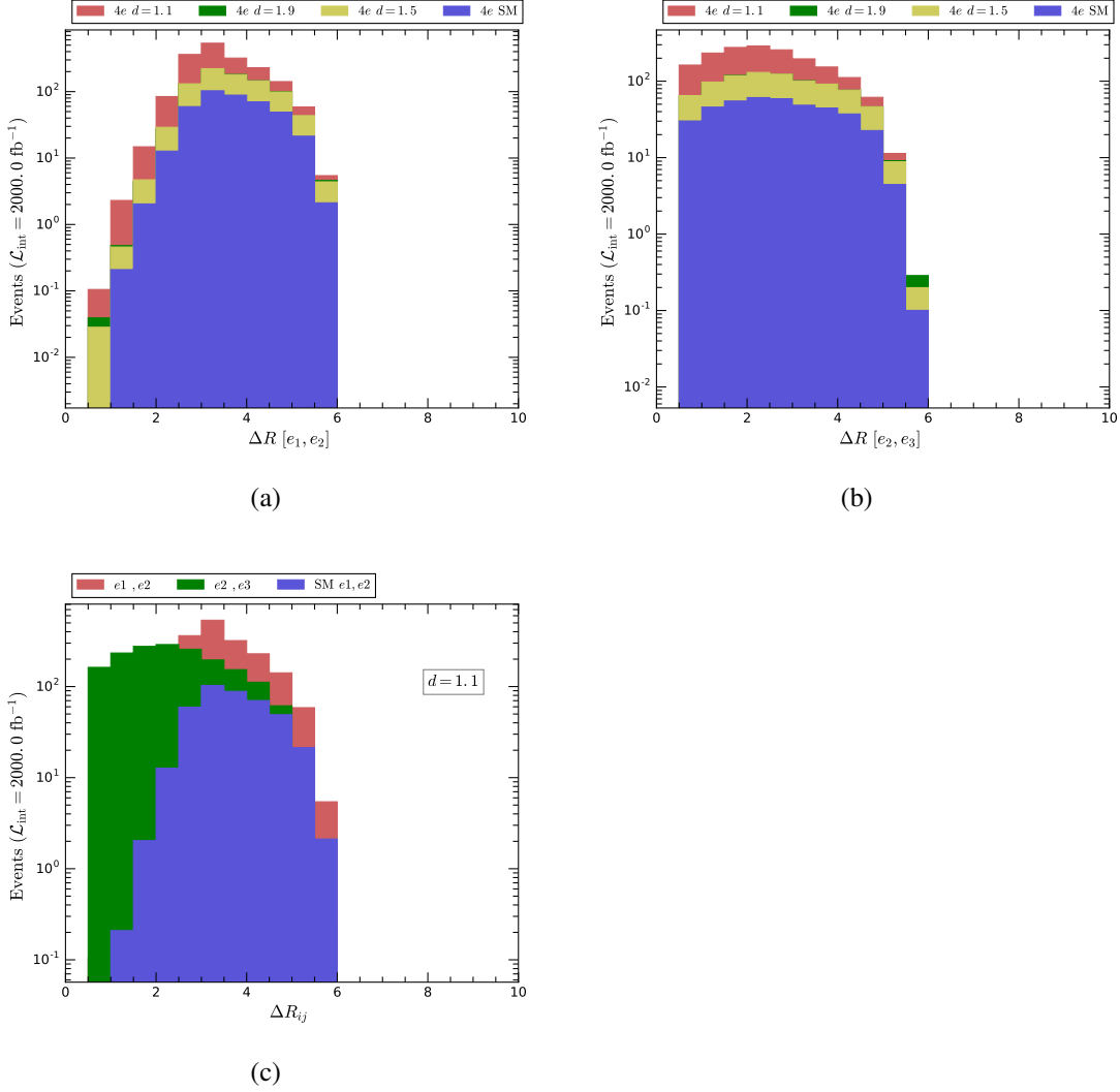
Figure 4.17: Various distributions of the process e^+e^- \rightarrow 4e in the framework of unparticle stuff with \sqrt{s} = 3 TeV at CLIC
