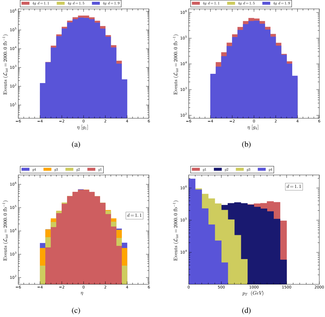
Figure 4.7: Various distributions of the process e^+e^- \rightarrow 4g in the framework of unparticle stuff with \sqrt{s} = 3 TeV at CLIC
