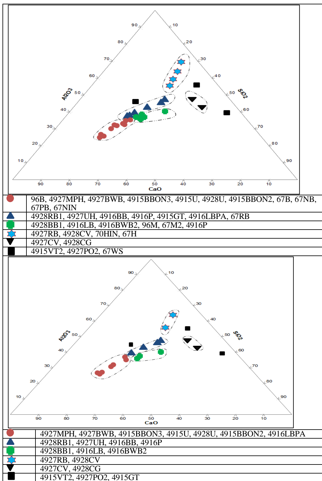
Figure 3.14. Distribution of samples according to some geochemical analysis (Martineau, 2007). Circles on the \text{Al}_2\text{O}_3/\text{CaO}/\text{SiO}_2 tri-plot graphs shows the results of cluster analysis as approximately. The upper graph includes all of the examples. Samples of Domuztepe are also shown In the chart below.
