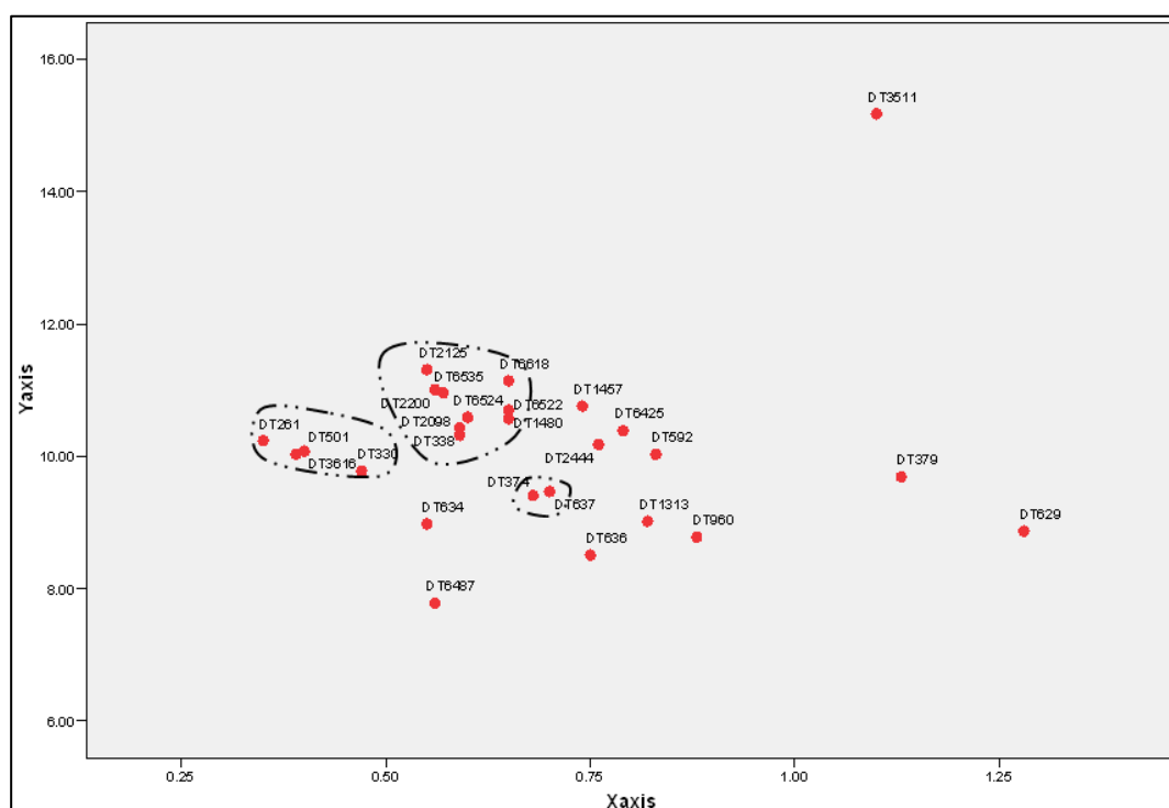
Figure 3.28. In the graph, according to x ( \log(\text{sum of REE})/\log \text{Cr} ) and y ( \text{sum of } \log \text{Cr} + \log \text{Zn} + \log \text{Fe} + \log \text{Co} / \log \text{Sc} ) axis data, the distribution of the samples are seen (Jones, 2007).
