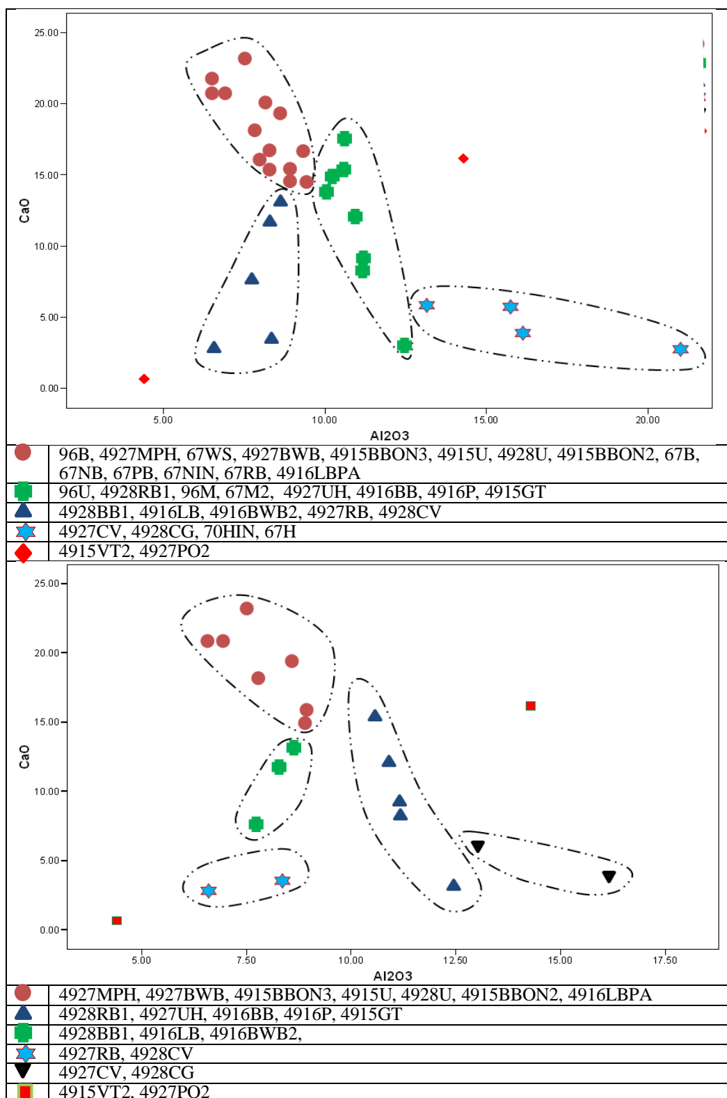
Figure 3.13. Distribution of samples according to some geochemical analysis (Barone G., 2005). Circles on the \text{Al}_2\text{O}_3/\text{CaO} graphs shows the results of cluster analysis as approximately. The upper graph includes all of the examples. Samples of Domuztepe are also shown In the chart below.
