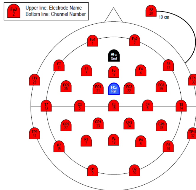
Figure 6: Easy cap 32 Channel Standard EEG Recording Cap: Electrodes with 6 mm central opening, extended 10/20-System placement.
