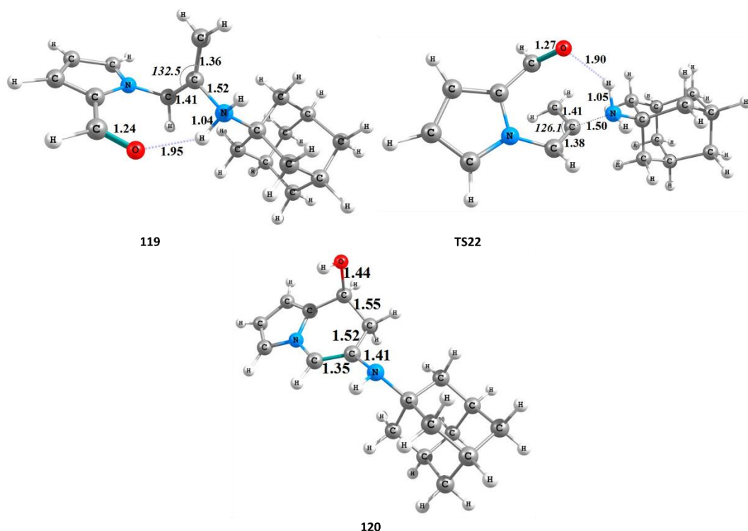
Figure 25. Optimized geometries of the stationary points of the second step for the formation of 120 at CPCM/B3LYP/6-31+G(d,p)//B3LYP/6-31+G(d,p) level in methanol. Distances are given in angstroms, angles are given in degrees
