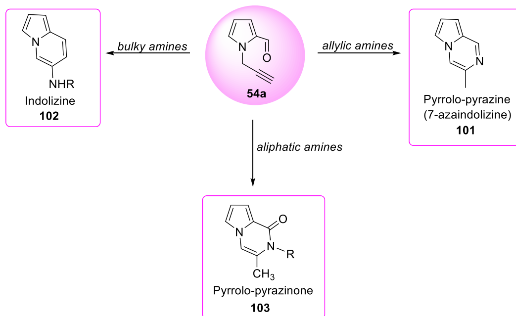
Scheme 30. Different skeletons obtained from N -propargyl carbaldehyde
