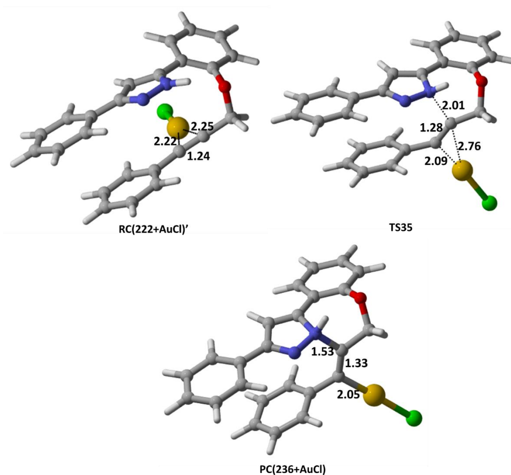
Figure 44. Optimized geometries for the 7- exo-dig reaction pathway at SMD(MeCN)/M06/6-31G(d)/LANL2DZ(f) level. Distances are given in angstroms. (carbon, grey; hydrogen, light grey; oxygen, red; nitrogen, blue; gold, yellow; chlorine, green)
