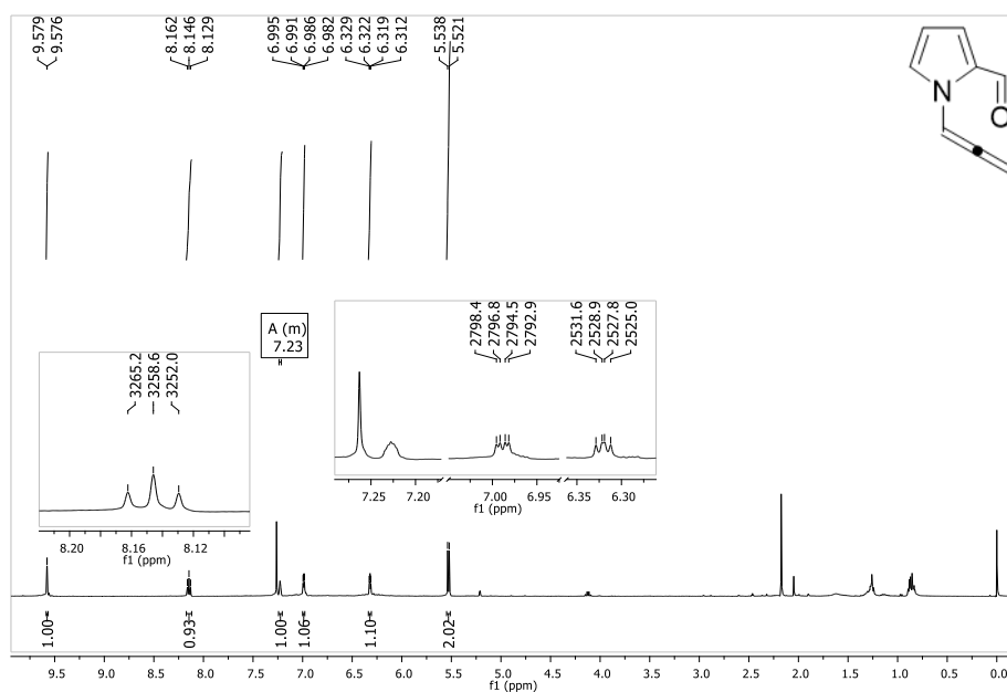
Figure 70. ^1\text{H} -NMR Spectrum of the Reaction of 1-(Prop-2-ynyl)-1 H -pyrrole-2-carbaldehyde with Propargylamine in Dry DMF
