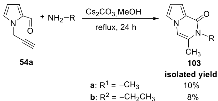
Scheme 38. Treatment of N -propargyl carbaldheyde 54a with aliphatic amines
