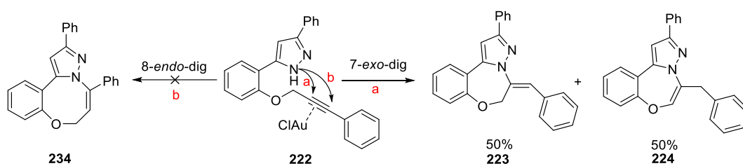
Scheme 81. Initial step for the hydroamination of 222
