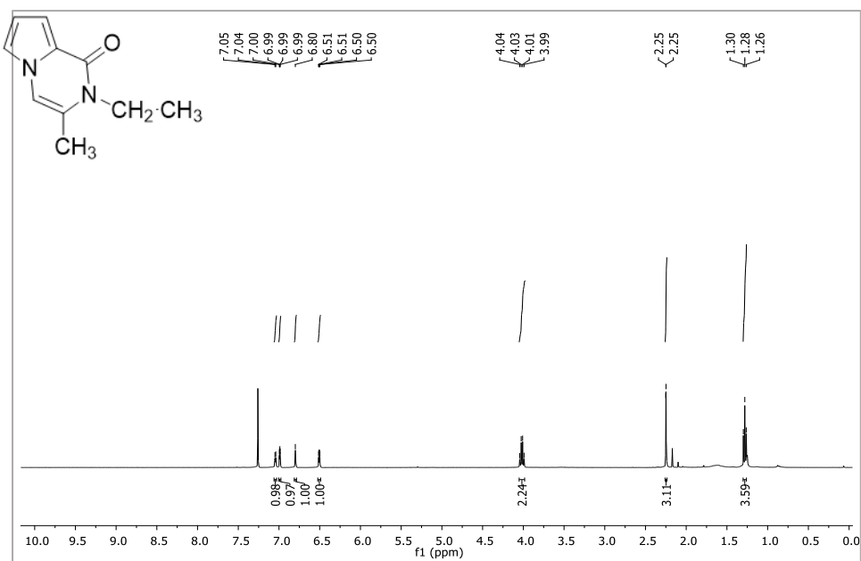
Figure 67. ^1\text{H} -NMR Spectrum of Compound 103b
