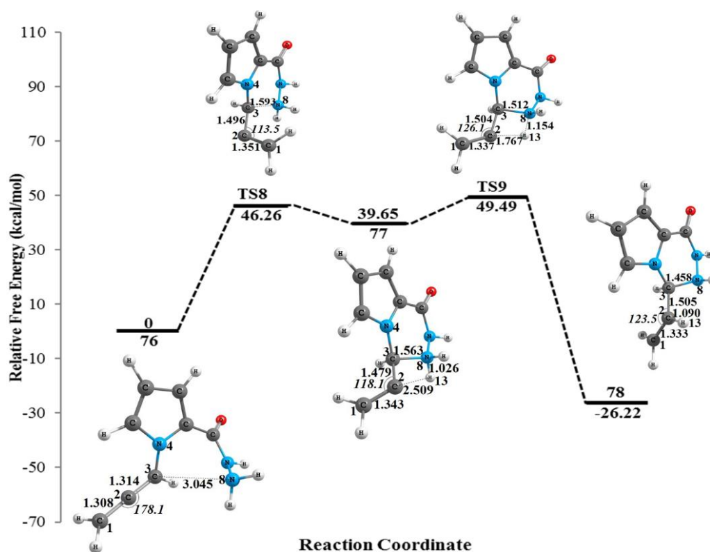
Figure 9. Potential energy surface for the formation of 78 at PCM/B3LYP/6-31+G(d,p)// B3LYP/6-31+G(d,p) level in methanol. Distances are given in angstroms; angles are given in degrees.
