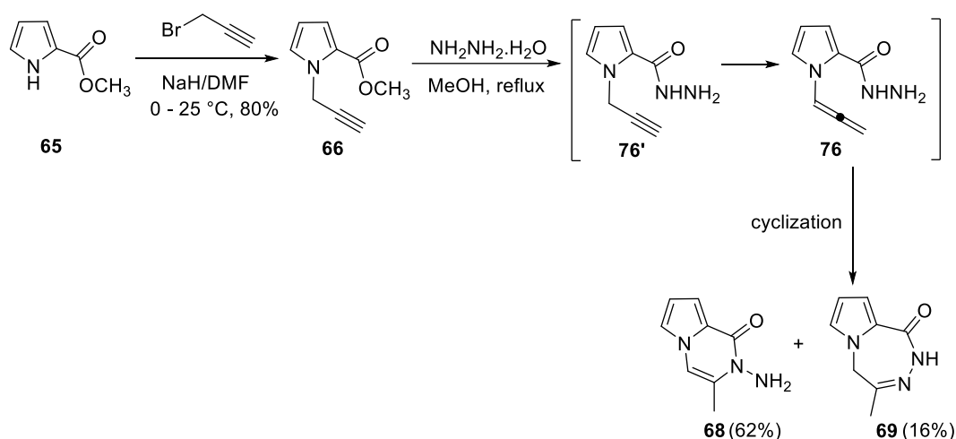
Scheme 99. Synthesis of pyrrolopyrazinone derivatives 69 starting from pyrrole ester 65
