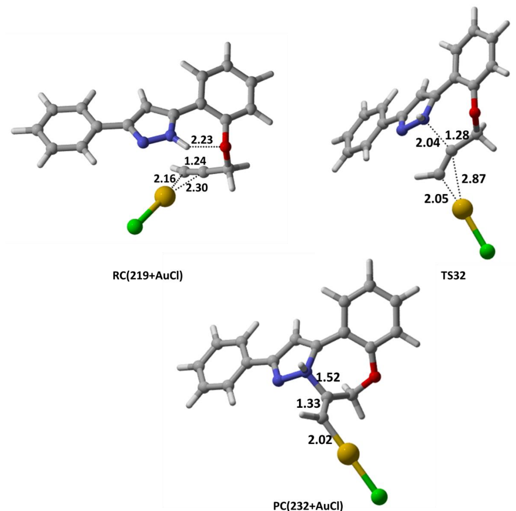
Figure 41. Optimized geometries for the 7- exo-dig reaction pathway at SMD(MeCN)/M06/6-31G(d)/LANL2DZ(f) level. Distances are given in angstroms. (carbon, grey; hydrogen, light grey; oxygen, red; nitrogen, blue; gold, yellow; chlorine, green)
