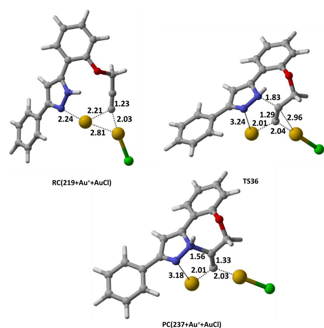
Figure 45. Optimized geometries for the dual gold catalysis at SMD(MeCN)/M06/6-31G(d)/LANL2DZ(f) level. Distances are given in angstroms. (carbon, grey; hydrogen, light grey; oxygen, red; nitrogen, blue; gold, yellow; chlorine, green)
