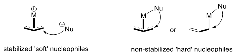
Scheme 86. Reaction mechanisms for stabilized and non-stabilized nucleophiles in asymmetric allylic substitution
