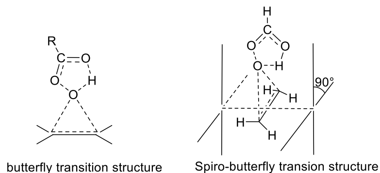
Figure 29. Proposed transition structures for the epoxidation of olefins
