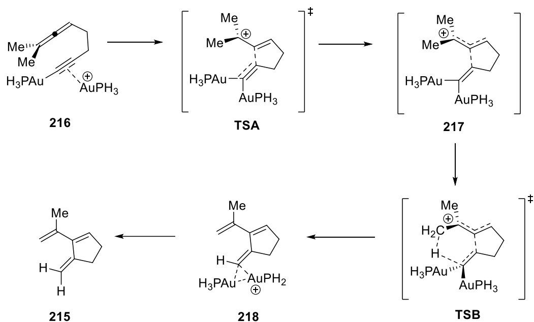
Scheme 74. Proposed mechanism for the formation of triene 215
