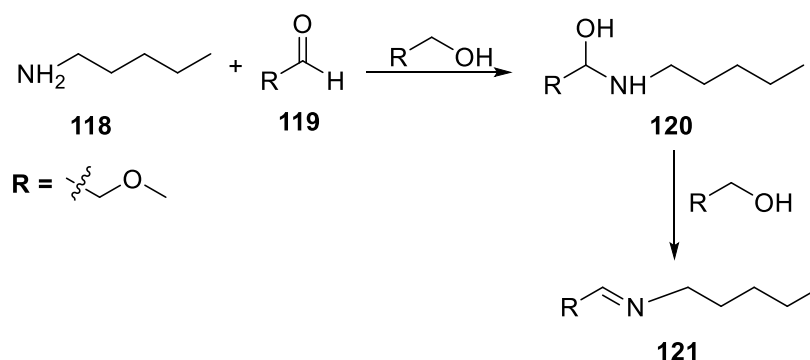
Scheme 42. Imine formation reaction starting from 2-methoxy-acetaldehyde 119 and pentyl amine 118
