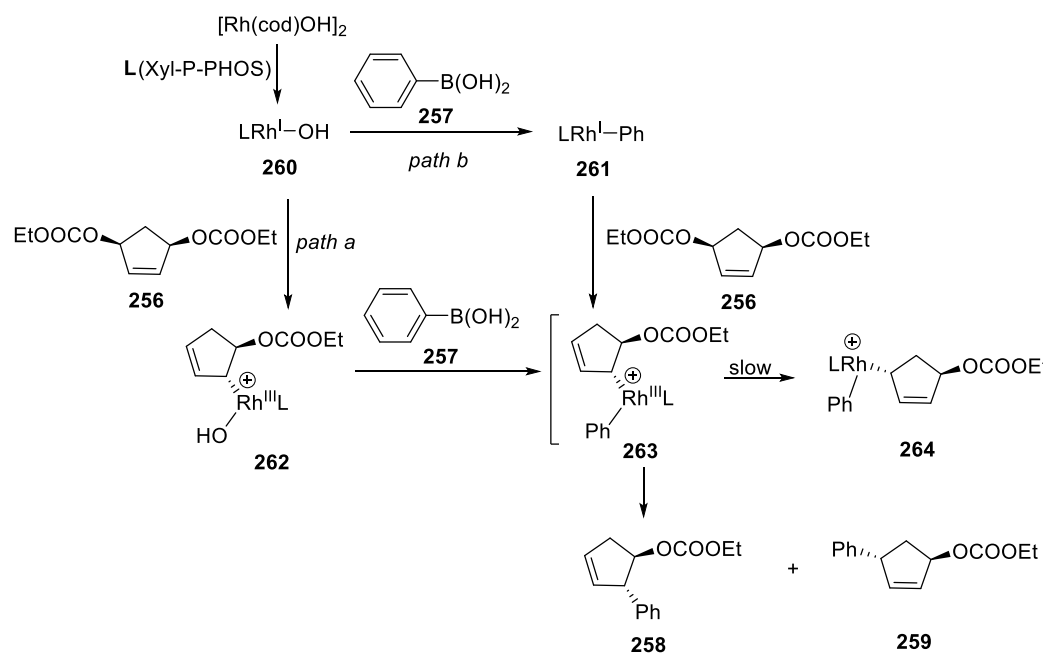
Scheme 91. Proposed mechanism for the Rh-catalyzed asymmetric allylic substitution reaction
