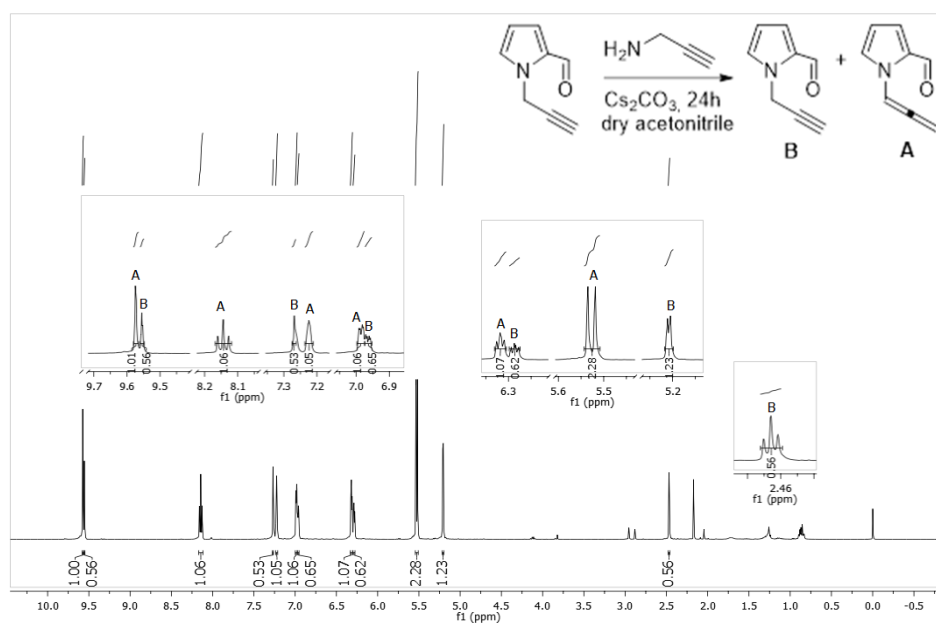
Figure 71. ^1\text{H} -NMR Spectrum of the Reaction of 1-(Prop-2-ynyl)-1 H -pyrrole-2-carbaldehyde with Propargylamine in Dry Acetonitrile
