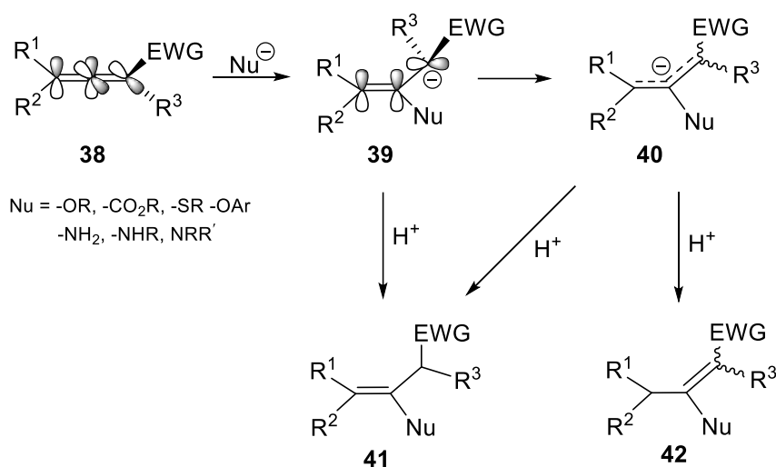
Scheme 13. Nucleophilic addition reaction of electron deficient allenes
