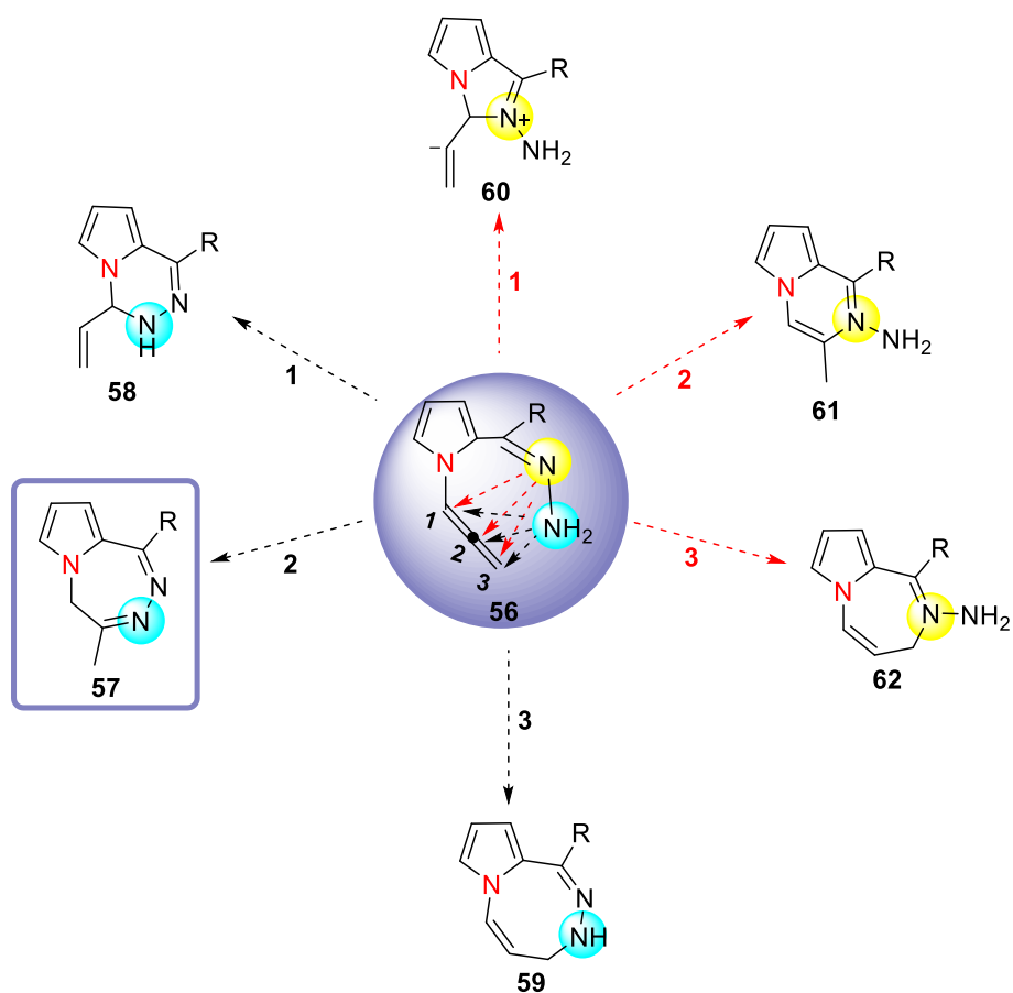
Scheme 18. Possible cyclization products
