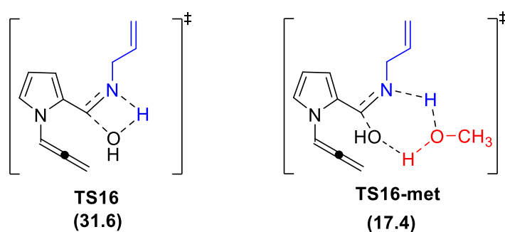
Scheme 44. Methanol-catalyzed and non-catalyzed transition states for the formation of 114 at CPCM/B3LYP/6-31+G(d,p)//B3LYP/6-31+G(d,p) level in methanol. The values in parenthesis represent the activation barriers of the corresponding step in kcal/mol.
