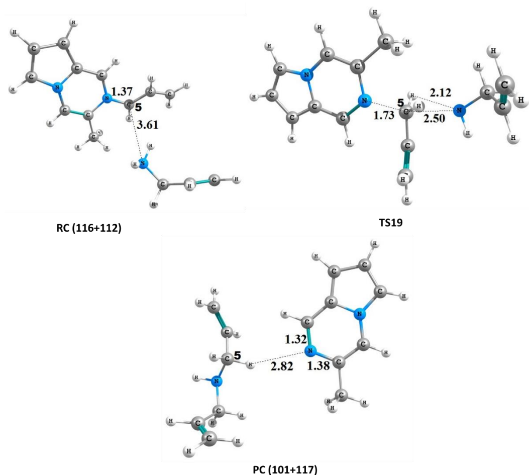
Figure 22. Optimized geometries of the stationary points of the formation of 3-methyl-pyrrolo[1,2- a ]pyrazine ( 101 ) at CPCM/B3LYP/6-31+G(d,p)//B3LYP/6-31+G(d,p) level in methanol. Distances are given in angstroms.
