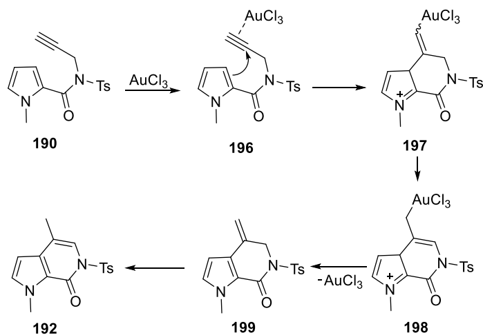
Scheme 68. Proposed mechanism for the formation of pyrrolopyridinone 192
