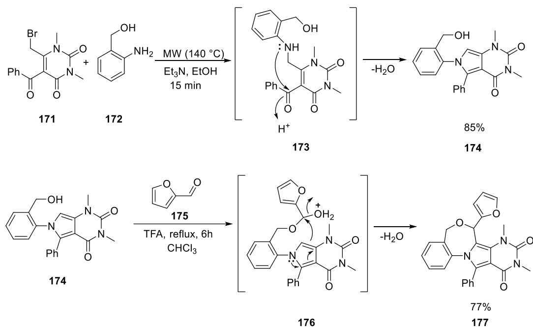
Scheme 59. Synthesis of 1,4-oxazepine derivative 177
