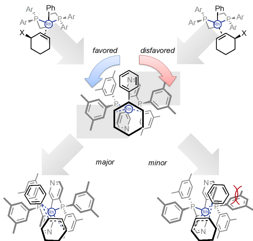
Figure 55. Proposed model for explaining the rate- and stereoselectivity-determining step for the asymmetric allylic arylation and critical transition states.
