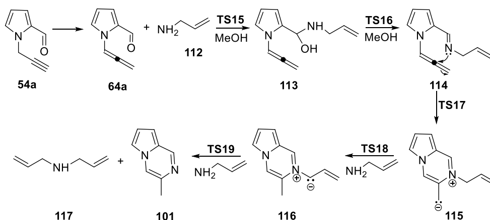
Scheme 41. Proposed mechanism for the formation of 3-methyl-pyrrolo[1,2- a ]pyrazine ( 101 )
