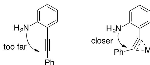
Scheme 63. Intramolecular hydroamination of alkynes with and without metal catalyst
