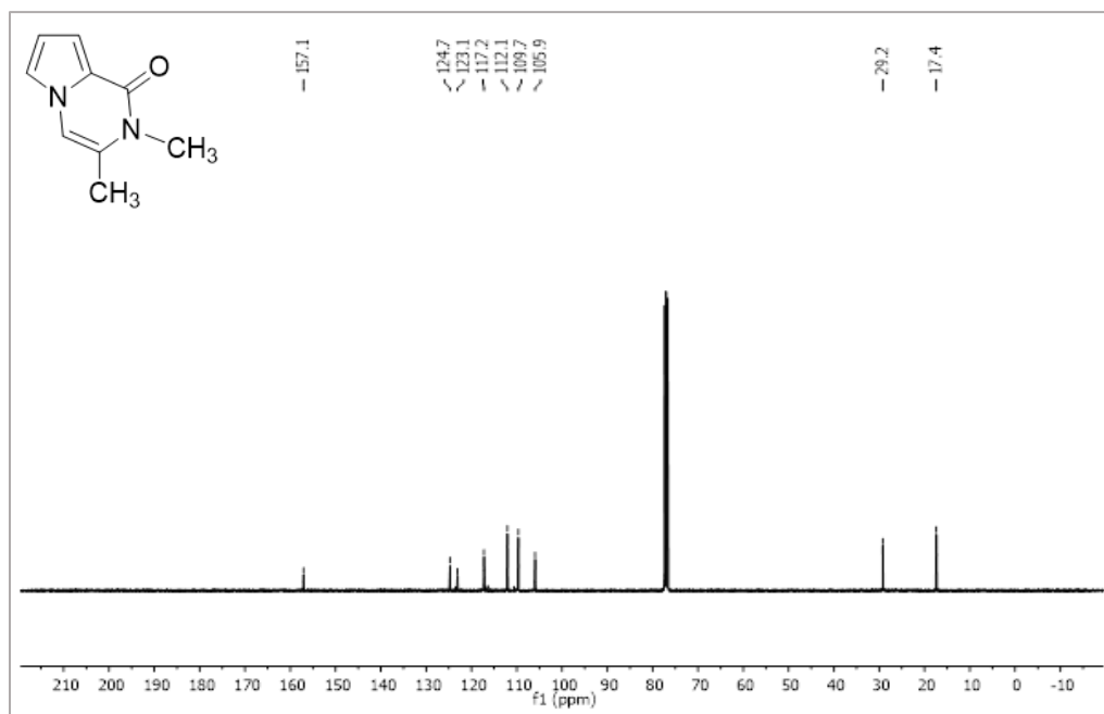
Figure 66. ^{13}\text{C} -NMR Spectrum of Compound 103a
