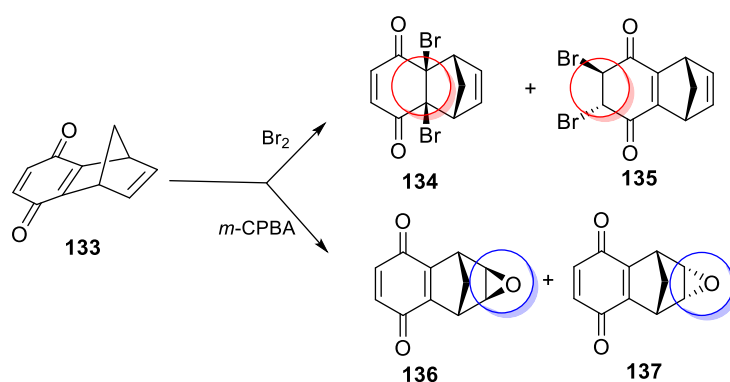
Scheme 51. Bromination and epoxidation of p -benzoquinone-fused norbornadiene 133
