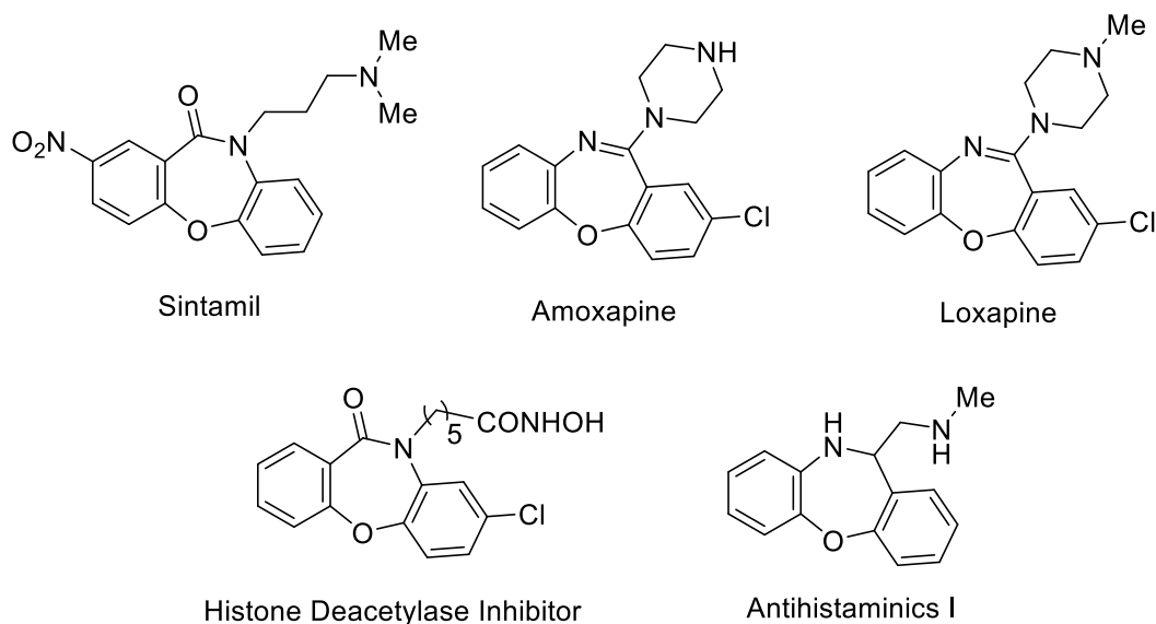
Figure 39. Structures of 1,4-oxazepine derivatives
