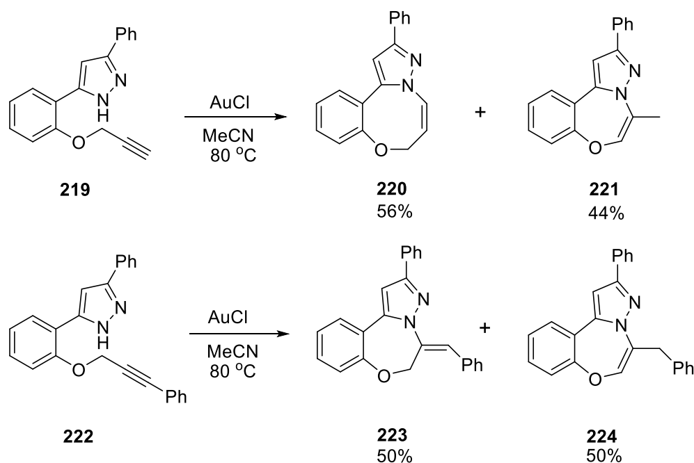
Scheme 102. Hydroamination reaction of terminal and internal alkynes 219 and 222 with AuCl
