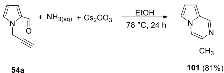
Scheme 32. The reaction of N -propargyl carbaldehyde 54a with ammonia
