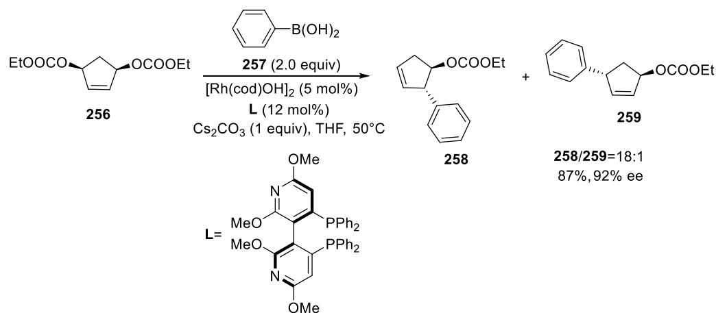
Scheme 90. Rh-catalyzed asymmetric allylic substitution with phenyl boronic acids
