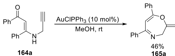
Scheme 57. Synthesis of 1,4-oxazepine derivative 165a
