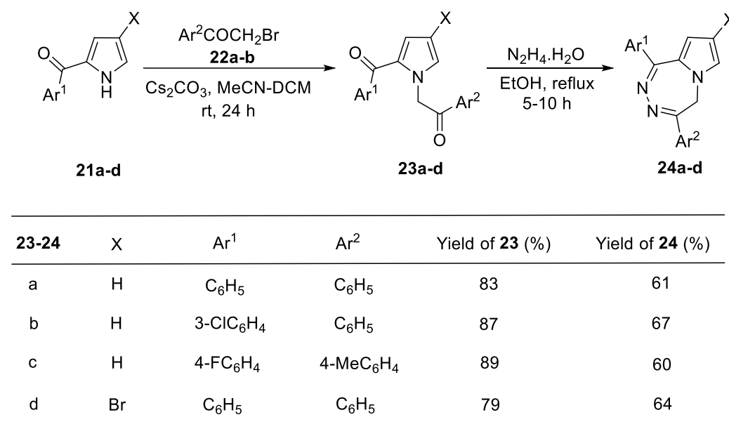
Scheme 7. Synthesis of pyrrolotriazepine derivative 24a-d
