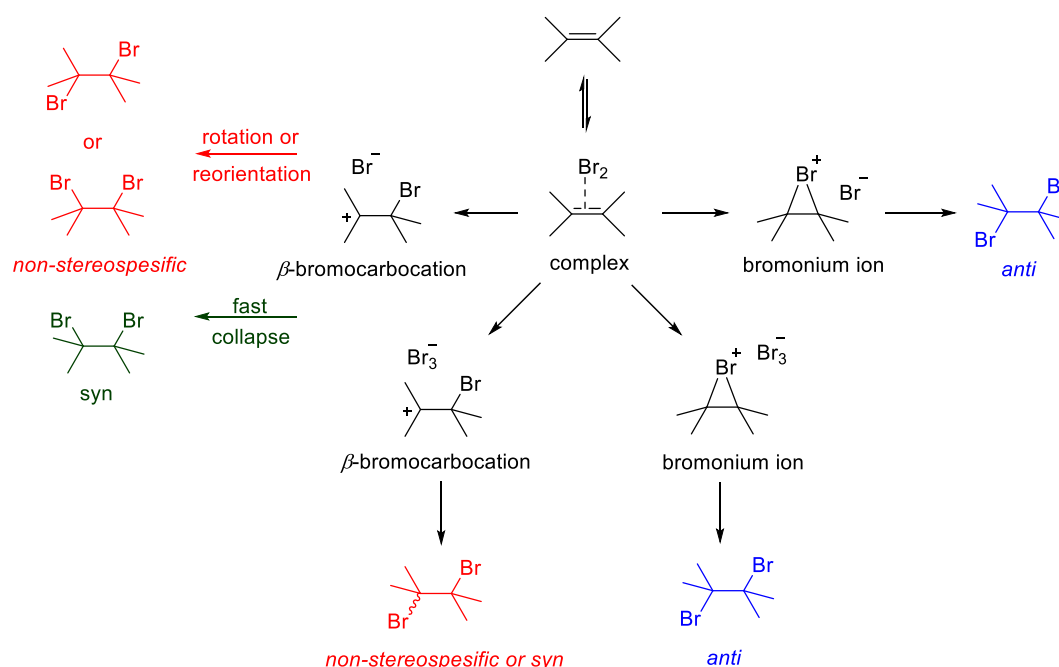
Scheme 48. Possible products for the bromination reaction
