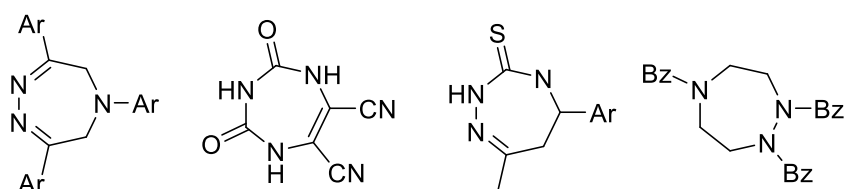
Figure 1. Examples of triazepine derivatives
