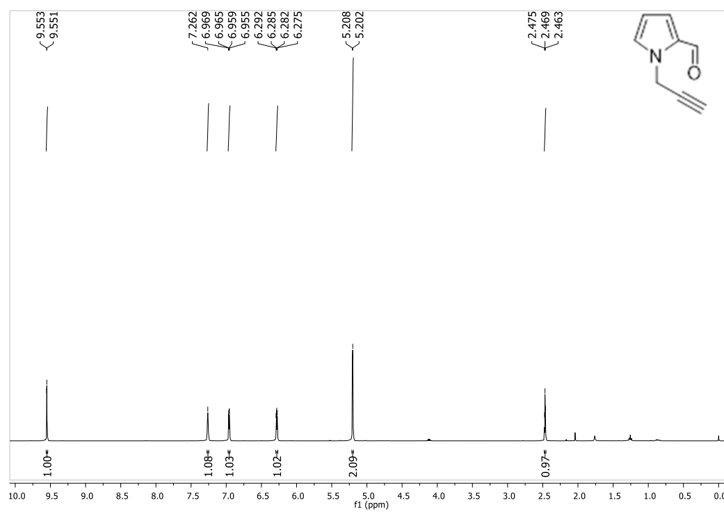
Figure 57. 1 H-NMR Spectrum of Compound 54a
