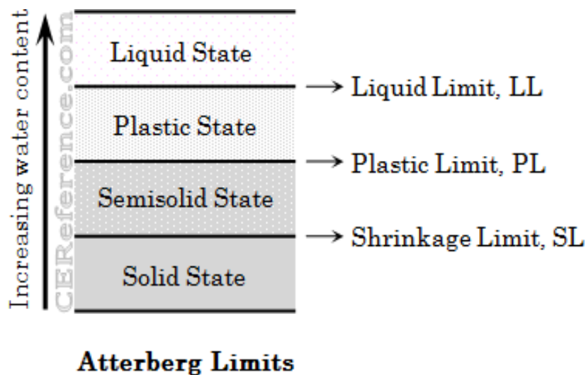
Figure 3.3 Fine-grained Soils States Boundaries According to water content and Atterberg Limits
