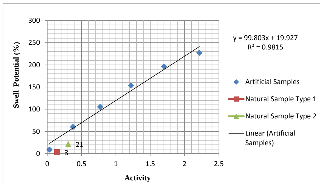
Figure 4.9 Swell Potential vs Activity
