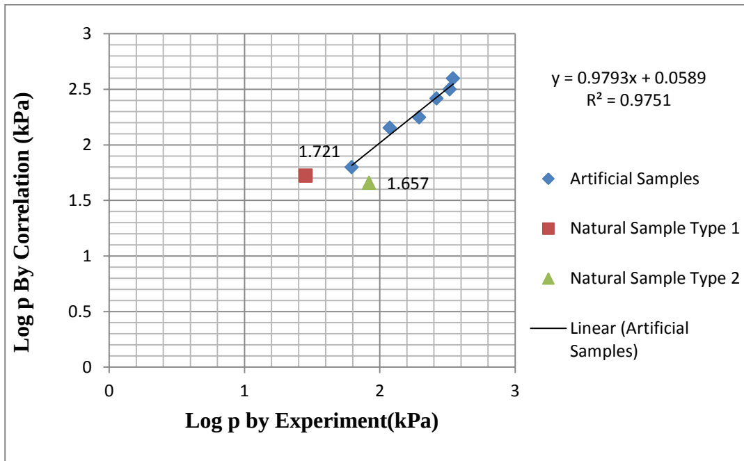
Figure 4.26 Comparison between experimental and predicted values of swelling pressure from model 3
