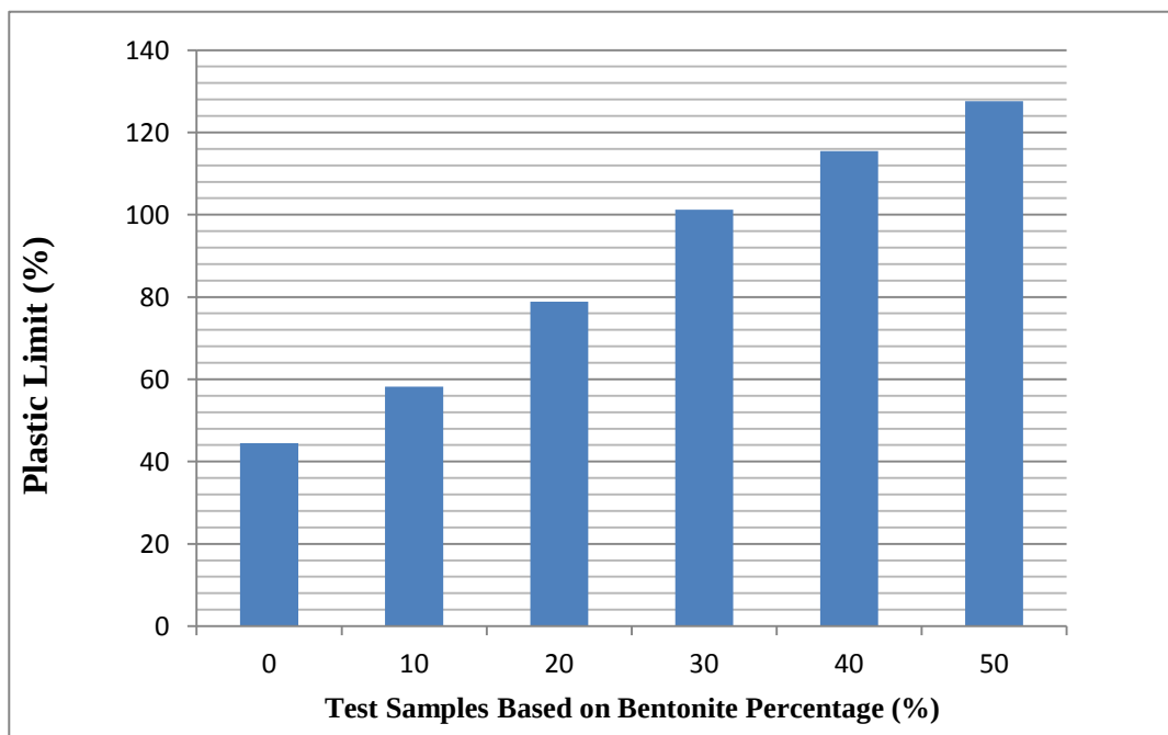
Figure 3.31 Plastic limit vs Sample types
