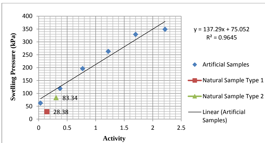
Figure 4.20 Swell Pressure vs Activity
