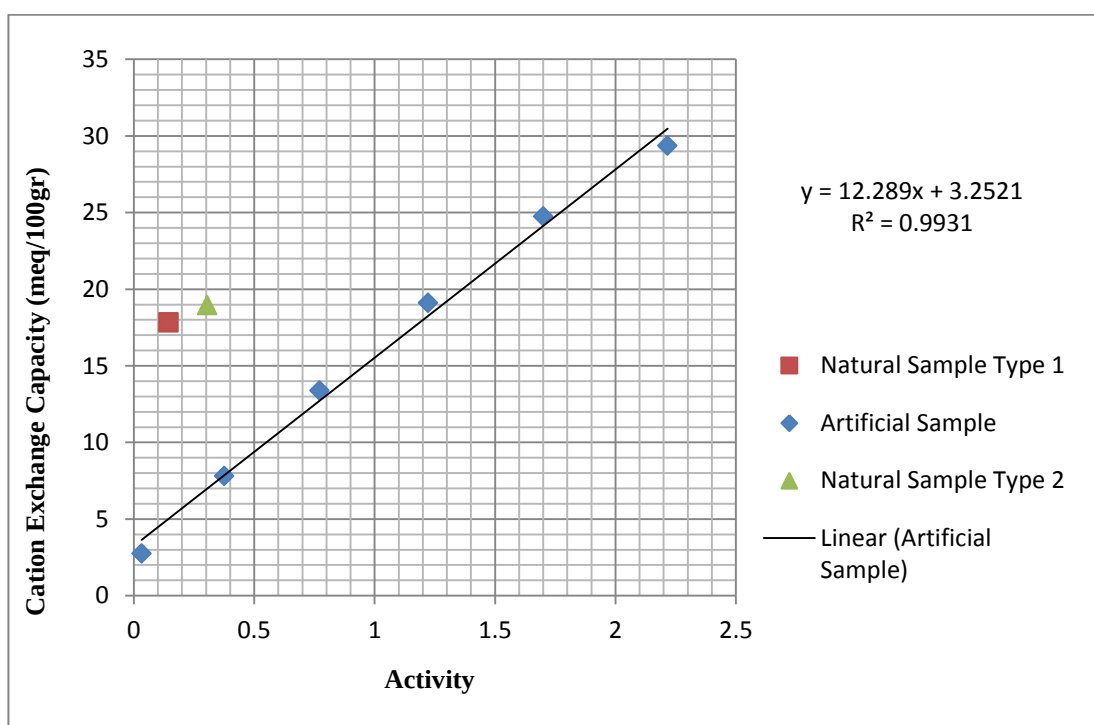
Figure B.8 C.E.C vs Activity
