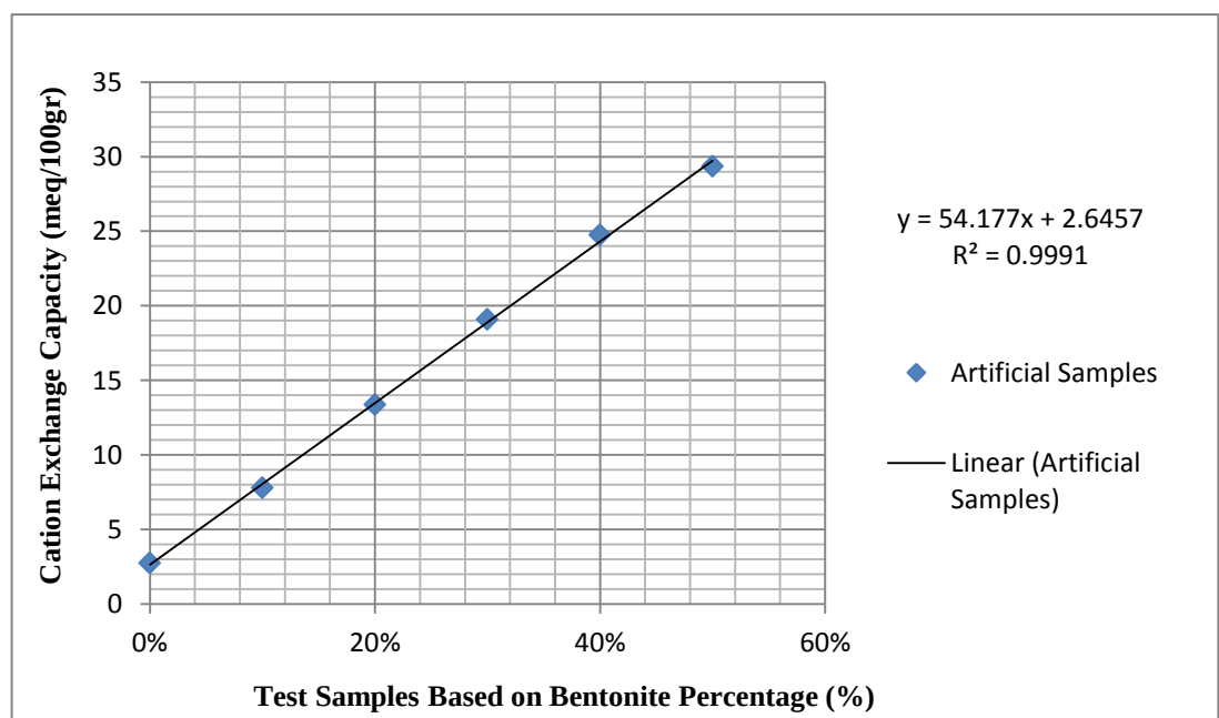
Figure B.5 C.E.C vs Test Samples
