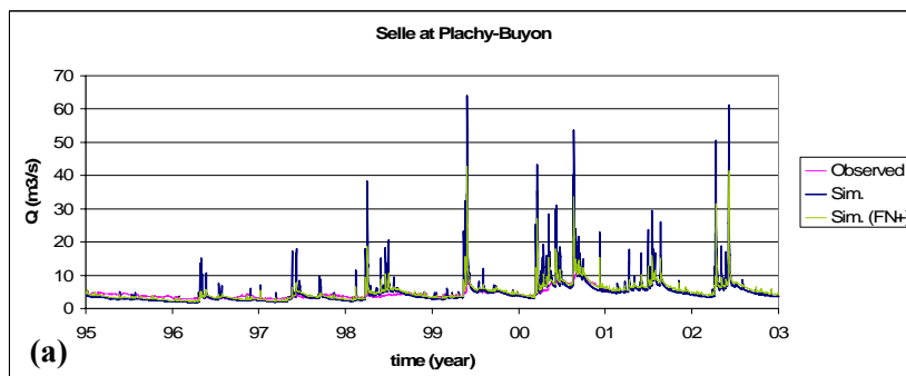
FIG. A. 3 The evolution of flow hydrograph of the Selle gauged at Plachy-Buyon ( 524 \text{ km}^2 ) during the calibration of MODSUR; a) increment of FN , b) decrement of C_{QR} , c) inclusion of NONSAT, d) calibration of parameters of Artificial Surfaces, e) calibration of parameters of Agricultural Zones.
