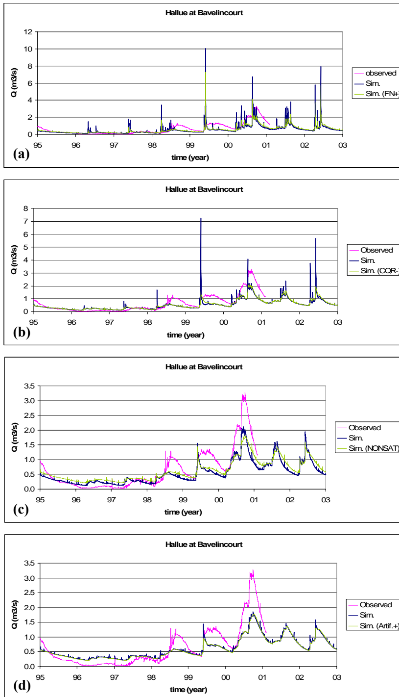
FIG. A. 4 The evolution of flow hydrograph of the Hallue gauged at Bavelincourt ( 115 \text{ km}^2 ) during the calibration of MODSUR; a) increment of FN , b) decrement of C_{QR} , c) inclusion of NONSAT, d) calibration of parameters of Artificial Surfaces, e) calibration of parameters of Agricultural Zones.
