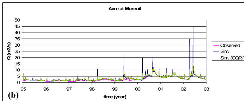
FIG. A. 2 The evolution of flow hydrograph of the Avre gauged at Moreuil (642 km 2 ) during the calibration of MODSUR; a ) increment of FN , b ) decrement of C_{QR} , c ) inclusion of NONSAT, d ) calibration of parameters of Artificial Surfaces, e ) calibration of parameters of Agricultural Zones.
