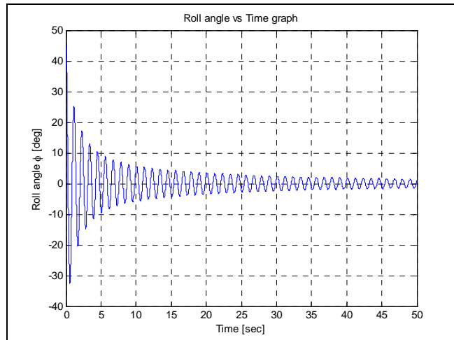
Figure 31 Roll angle
