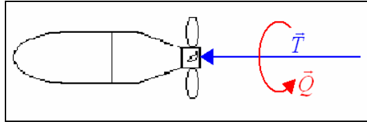
Figure 10 Torque and Force of Thruster
