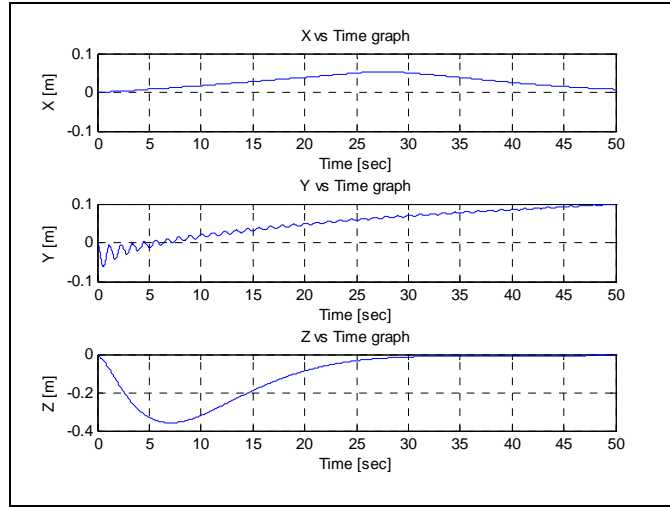
Figure 32 Vehicle Positions
