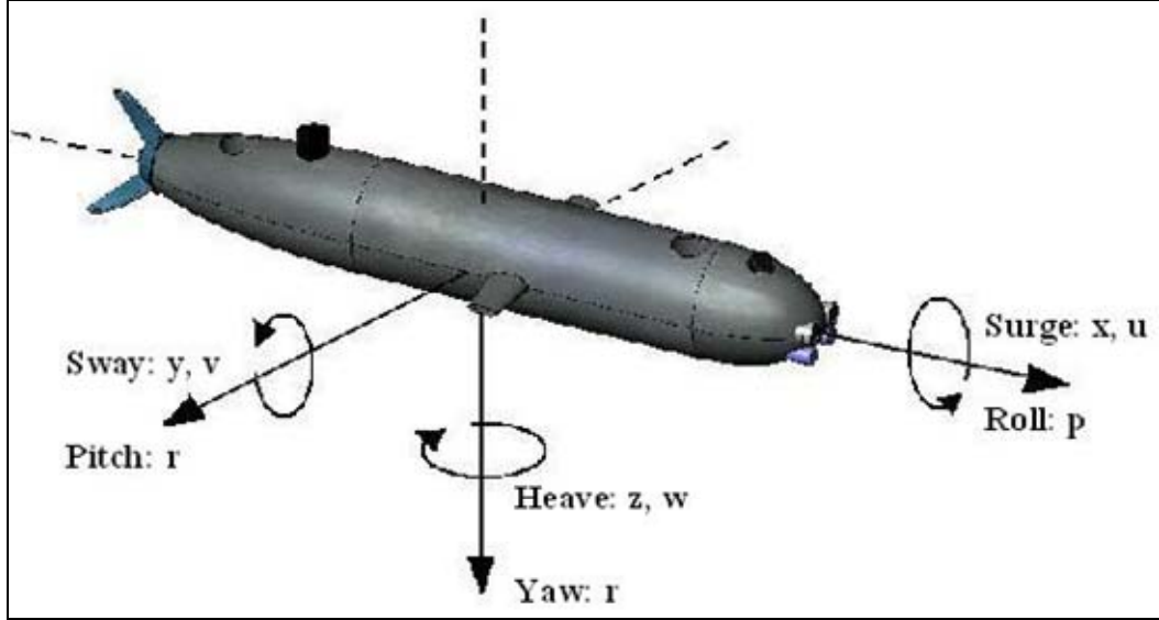
Figure 4 Body Fixed Coordinate system
