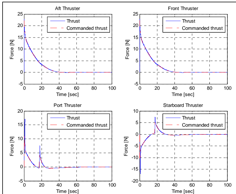
Figure 27 Thrust Forces
