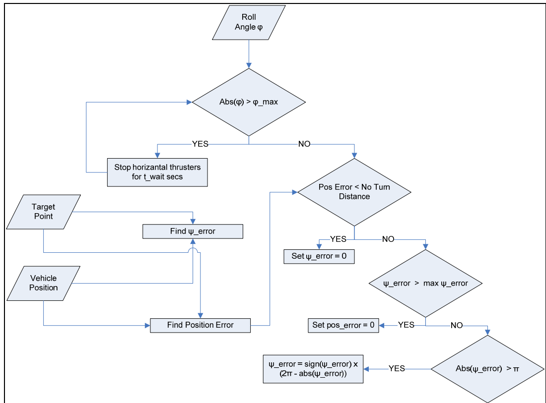
Figure 14 Flow diagram of the autopilot
