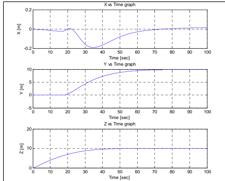
Figure 25 Earth fixed coordinates of the vehicle
