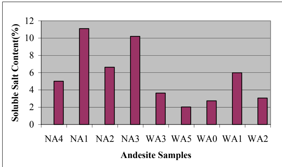
Figure 3.5 Distribution of soluble salts in andesite samples taken from north and west elevations of Gençkapı Gate
