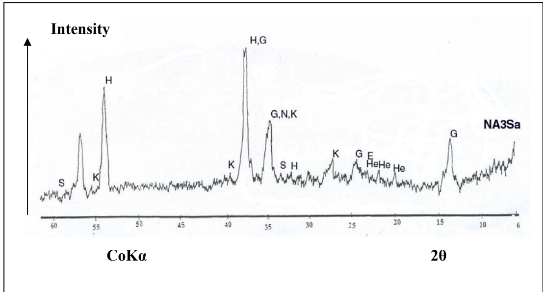
Figure 3.8 XRD pattern of salt sample extracted from andesite sample NA3: H :Halite ( \text{NaCl} ); K : Niter( \text{KNO}_3 ); S : Sylvite ( \text{KCl} ); G :Gypsum ( \text{CaSO}_4 \cdot 2\text{H}_2\text{O} ); He :Hexahydrite ( \text{MgSO}_4 \cdot 6\text{H}_2\text{O} ); E :Epsomite( \text{MgSO}_4 \cdot 6\text{H}_2\text{O} ); N :Sodaniter( \text{NaNO}_3 )
