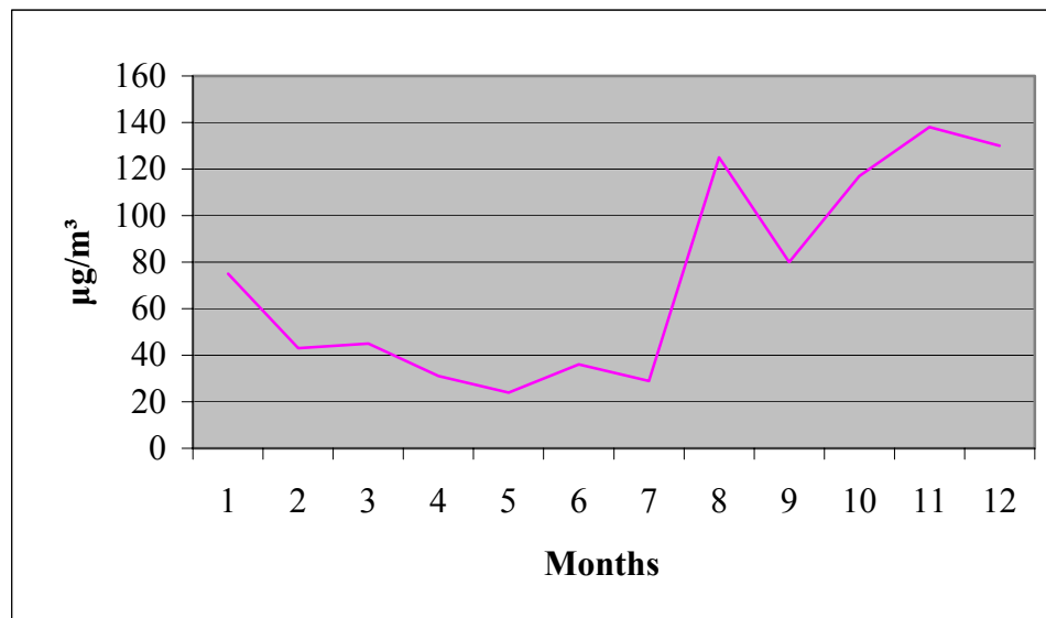
Figure 1.8 Average NO concentrations in the Ankara atmosphere in 2003 (IHP, 2003)
